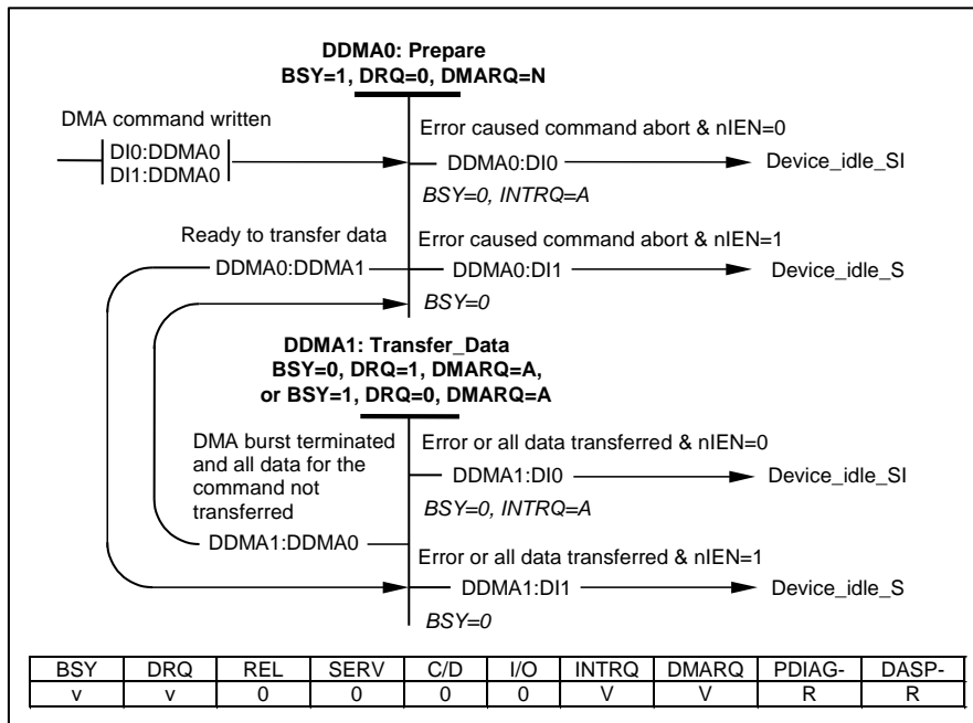
Figure 52 – Device DMA state diagram
