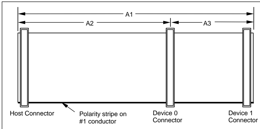
Figure 8 – 40-conductor cable configuration
