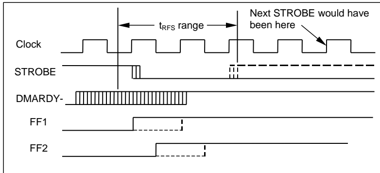
Figure 111 - DMARDY- to final STROBE t_{RFS} synchronization
