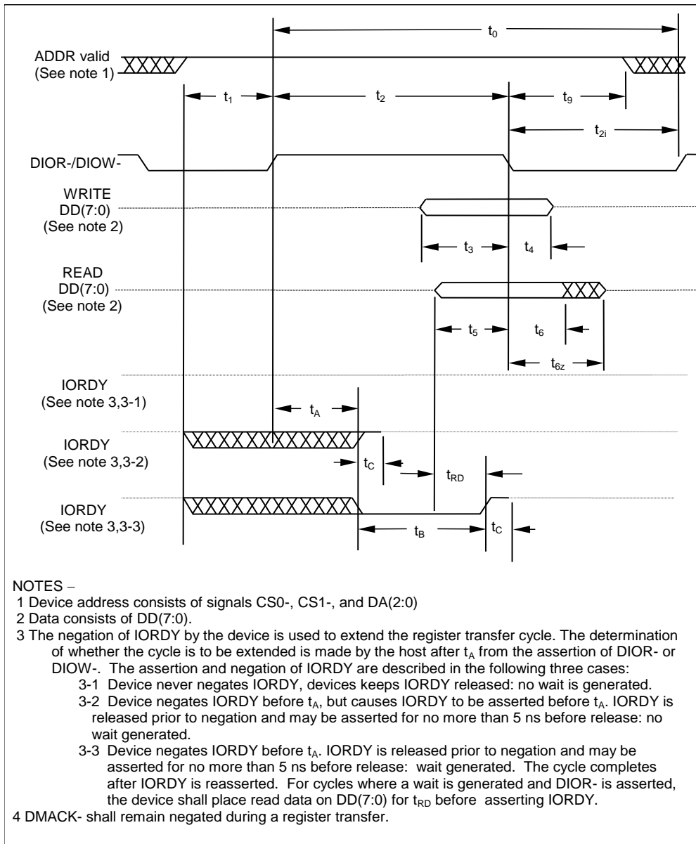
Figure 65 – Register transfer to/from device
