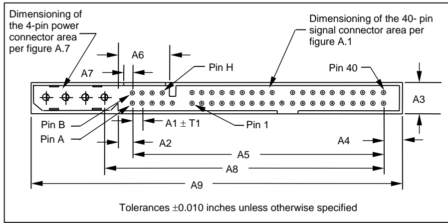
Figure 14 – Unitized connector
