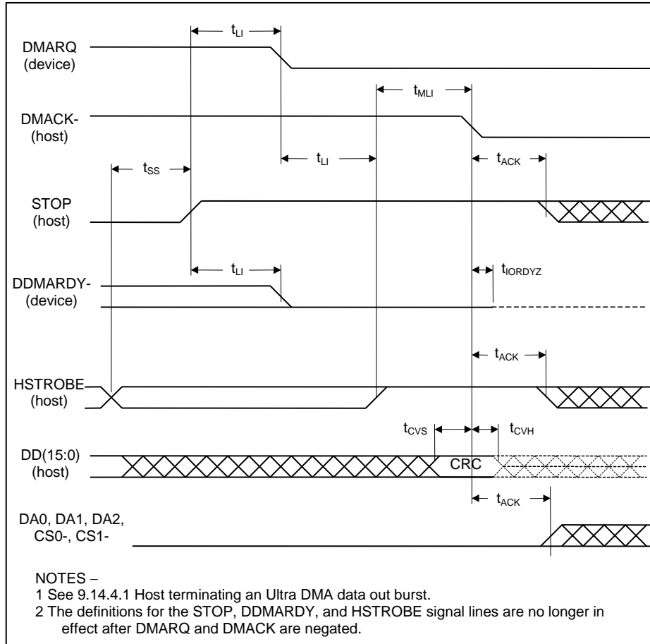
Figure 79 – Host terminating an Ultra DMA data-out burst
