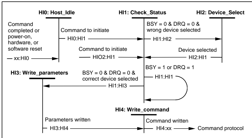
Figure 41 – Host bus idle state diagram
