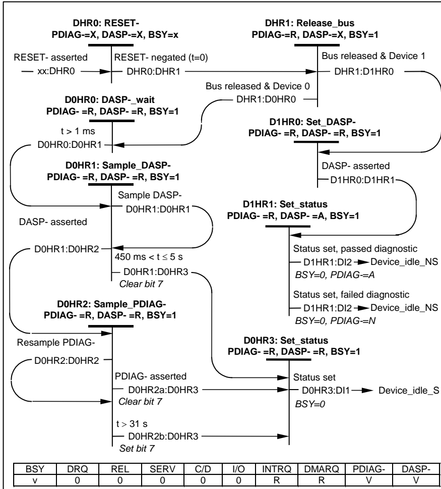
Figure 37 – Device power-on or hardware reset state diagram
