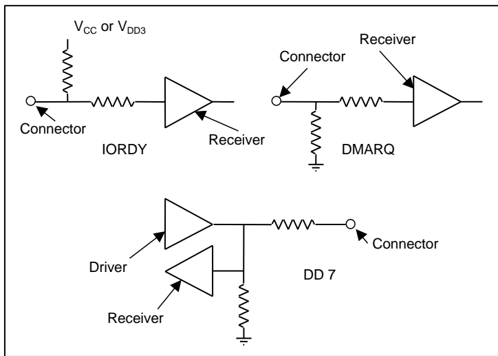
Figure 4 – Ultra DMA termination with pull-up or pull-down
