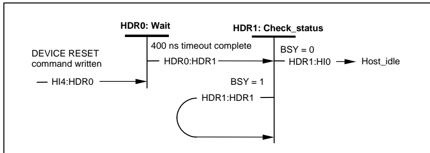
Figure 62 – Host DEVICE RESET command state diagram
