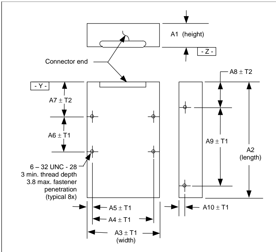
Figure 19 – 3.5" form factor
