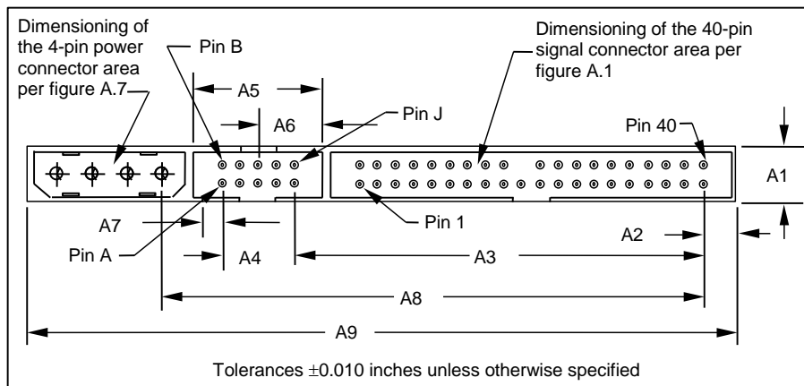
Figure 15 – Unitized connector
