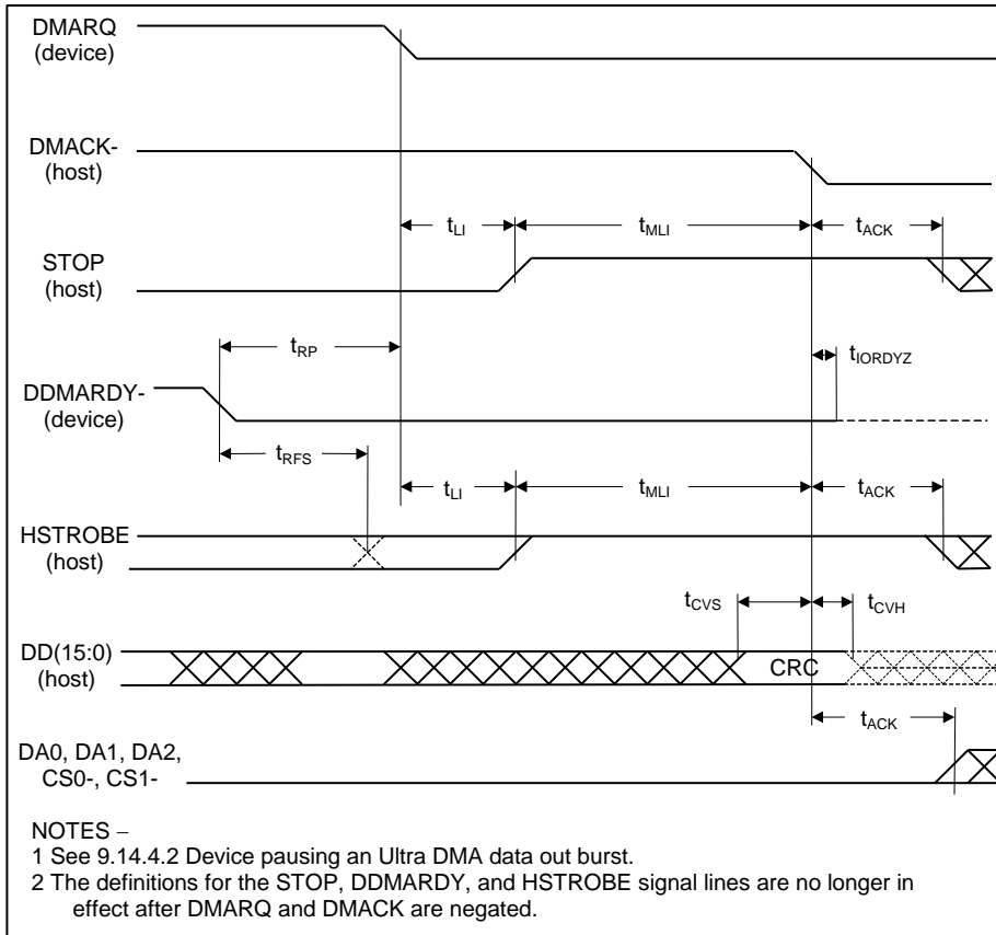
Figure 80 – Device terminating an Ultra DMA data-out burst
