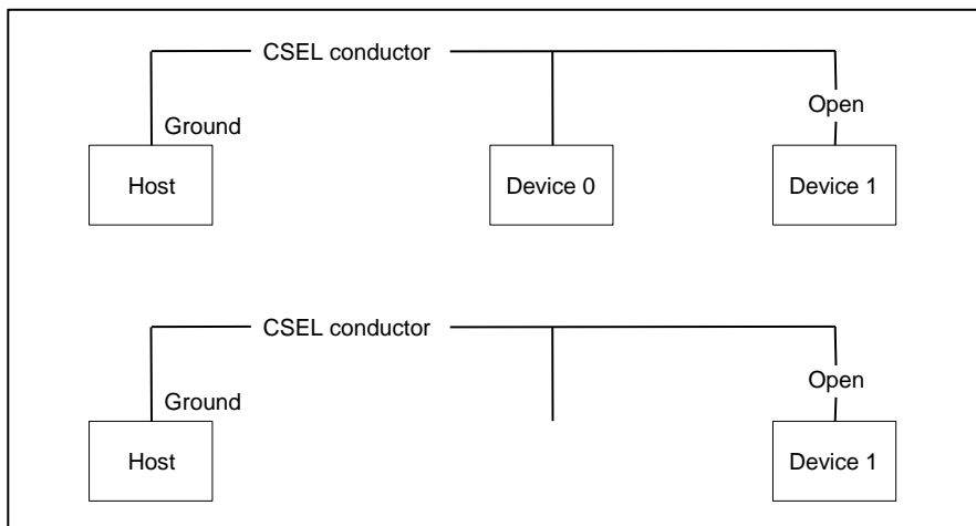
Figure 29 – Cable select example
