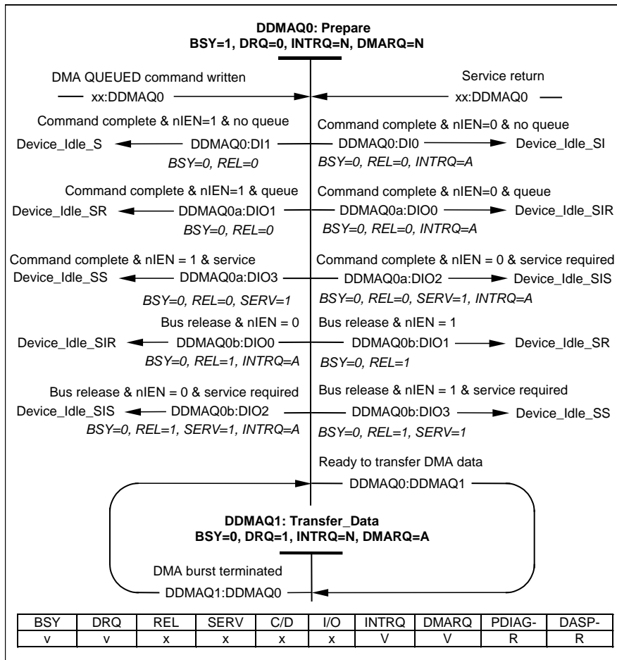
Figure 58 – Device DMA QUEUED command state diagram
