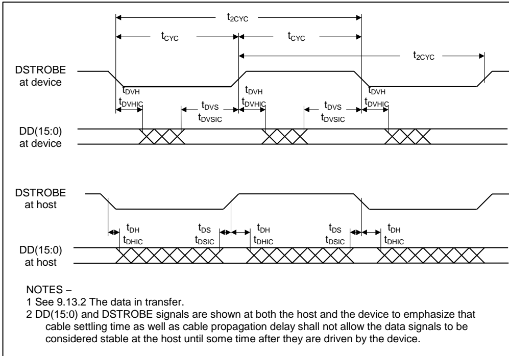
Figure 72 – Sustained Ultra DMA data-in burst
