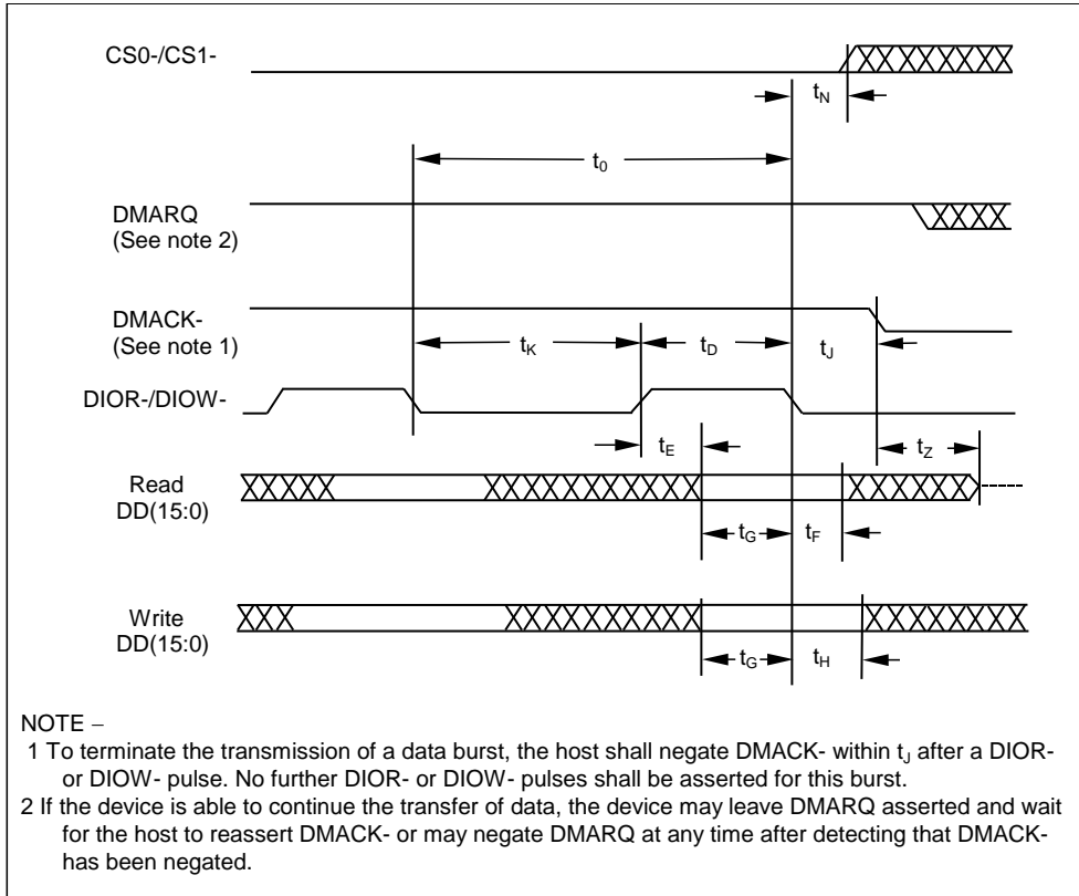
Figure 70 – Host terminating a Multiword DMA data burst
