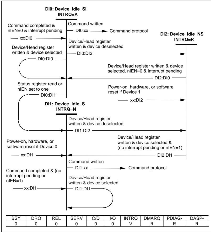
Figure 43 – Device bus Idle state diagram
