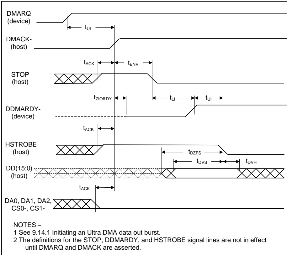
Figure 76 – Initiating an Ultra DMA data-out burst
