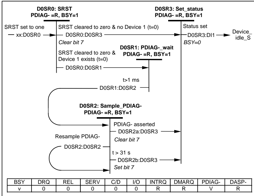
Figure 39 – Device 0 software reset state diagram
