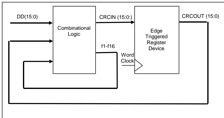
Figure 64 – Example Parallel CRC generator
