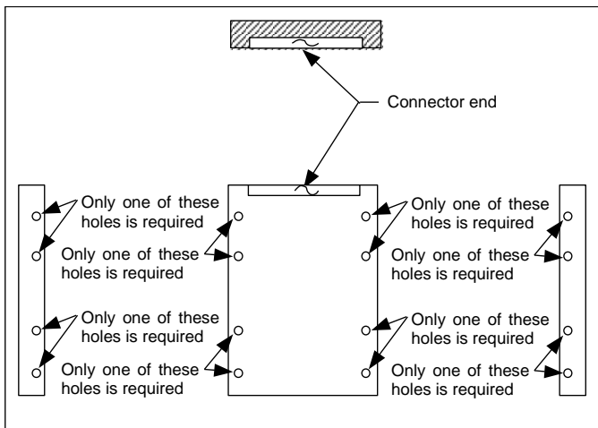
Figure 21 – 2.5" form factor mounting holes
