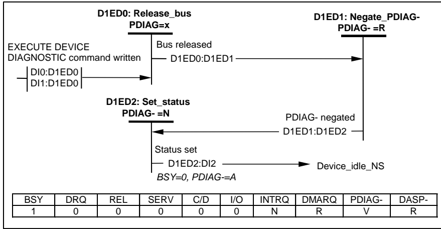
Figure 61 – Device 1 device diagnostic command state diagram
