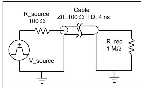
Figure 82 - A transmission line with perfect source termination
