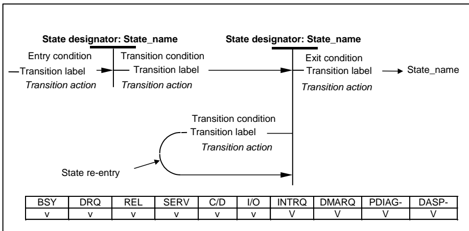
Figure 2 – State diagram convention
