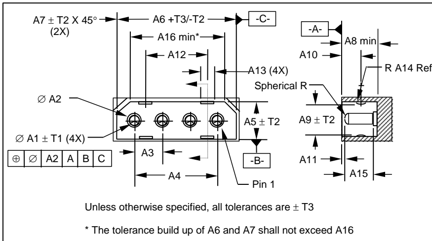
Figure 12 – Device 4-pin power header
