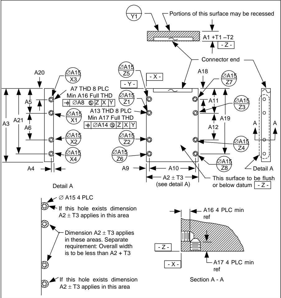
Figure 20 – 2.5" form factor
