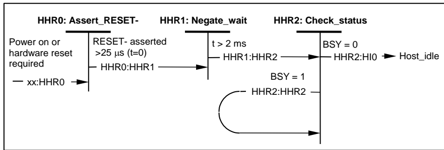
Figure 36 – Host power-on or hardware reset state diagram
