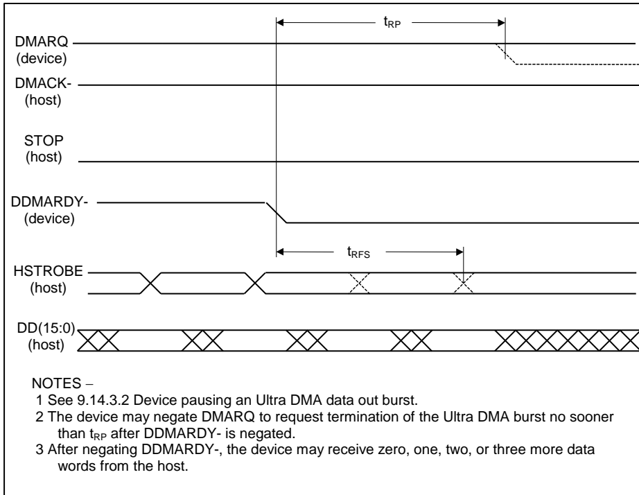
Figure 78 – Device pausing an Ultra DMA data-out burst
