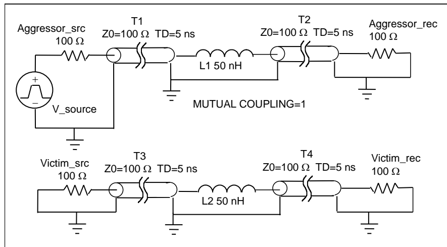
Figure 93 - Model of inductive coupling
