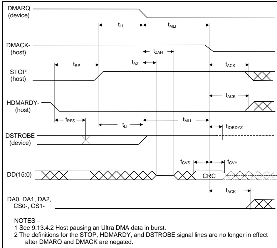
Figure 75 – Host terminating an Ultra DMA data-in burst
