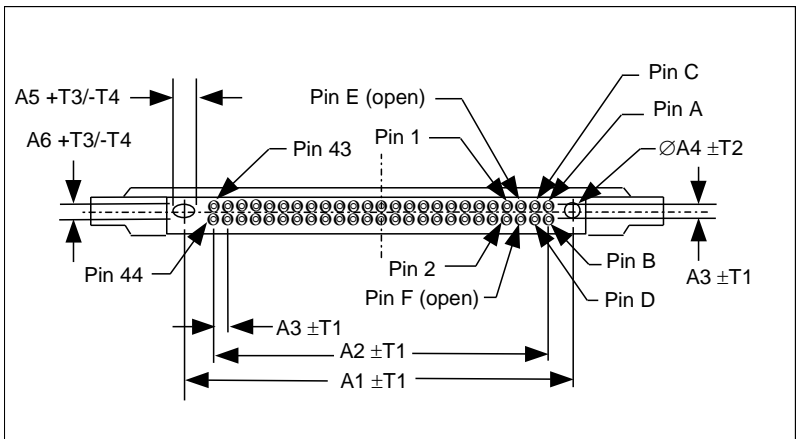
Figure 17 – 1.8 inch 3.3V parallel connector
