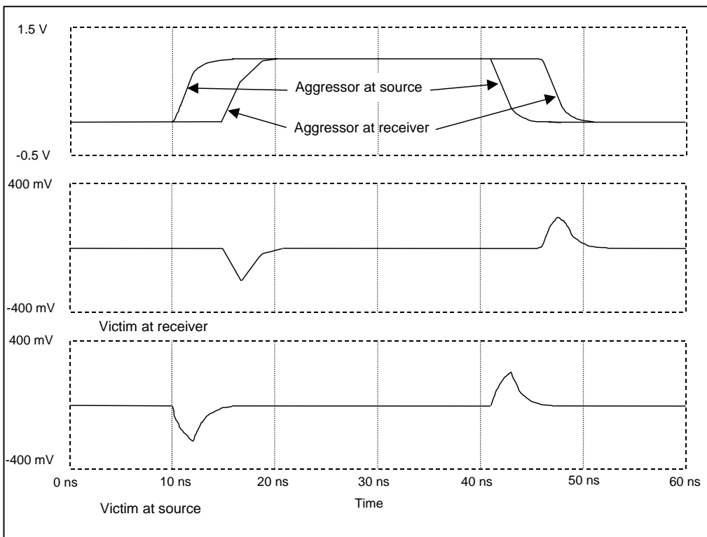
Figure 102 - Waveforms resulting from ground bounce (at transmitter and receiver of aggressor and victim)
