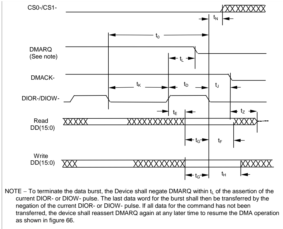
Figure 69 – Device terminating a Multiword DMA data burst
