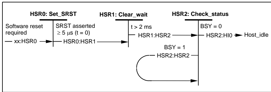
Figure 38 – Host software reset state diagram
