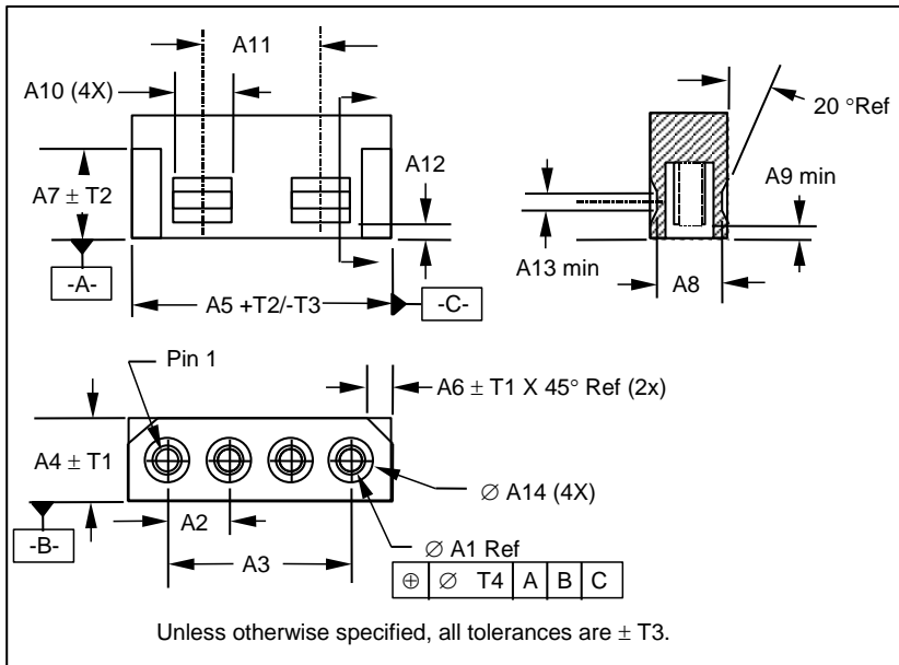
Figure 13 – 4-pin power cable connector
