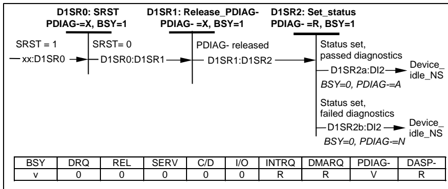
Figure 40 – Device 1 software reset state diagram
