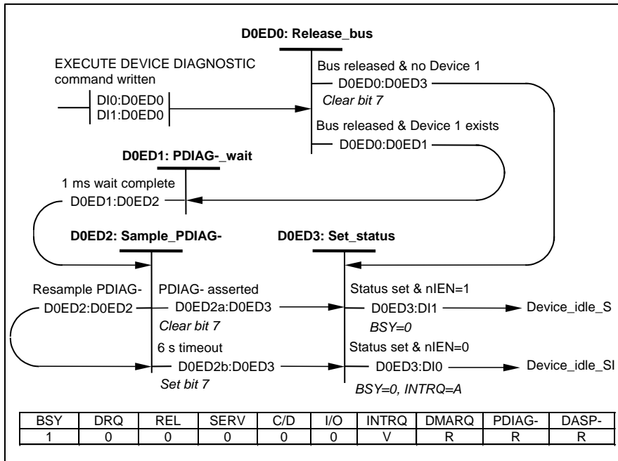
Figure 60 – Device 0 device diagnostic state diagram
