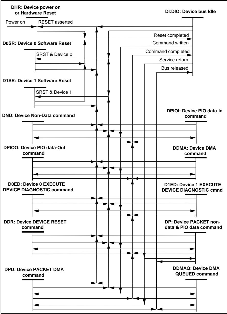
Figure 35 – Overall device protocol state sequence
