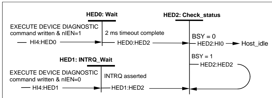
Figure 59 – Host EXECUTE DEVICE DIAGNOSTIC state diagram
