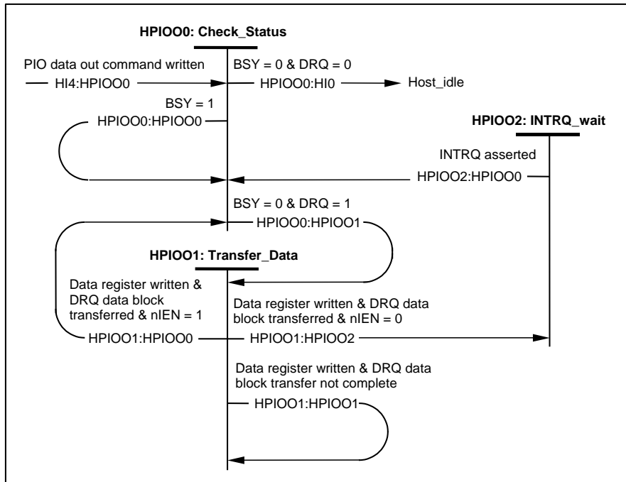
Figure 49 – Host PIO data-Out state diagram
