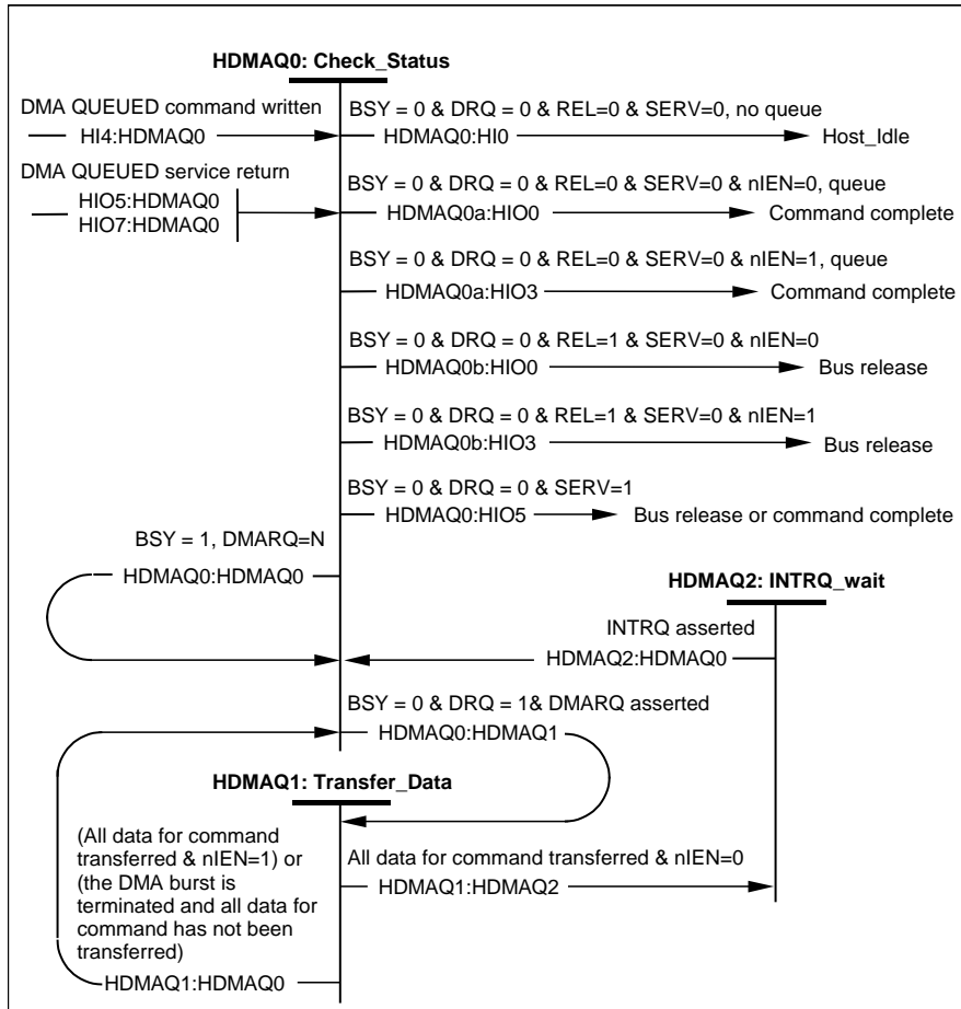
Figure 57 – Host DMA QUEUED state diagram
