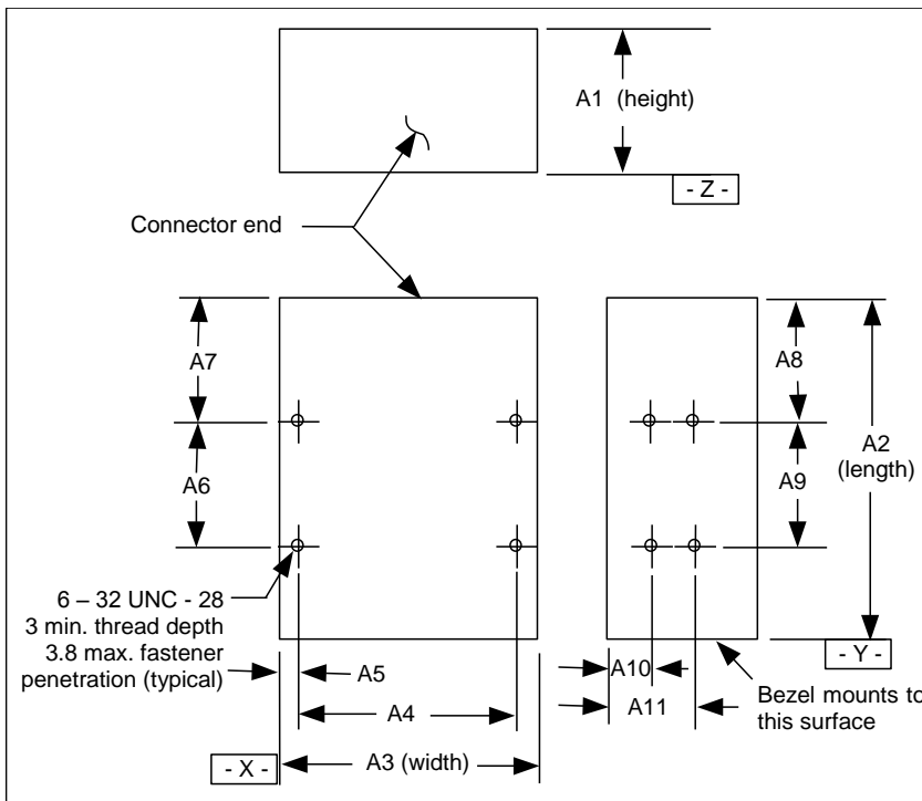
Figure 27 – 5.25 inch CD-ROM form factor
