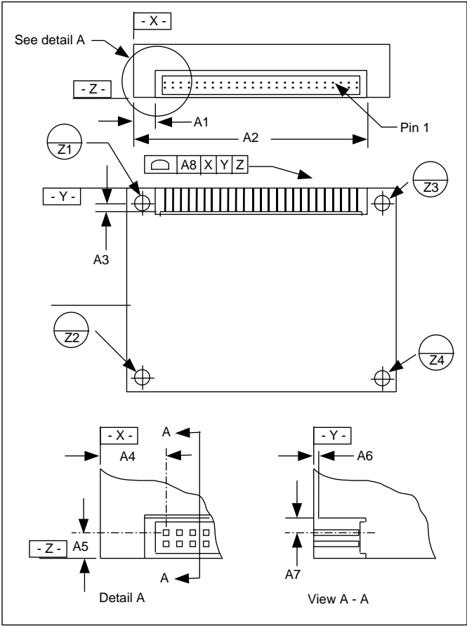
Figure 24 – 1.8 inch 5V parallel form factor connector location
