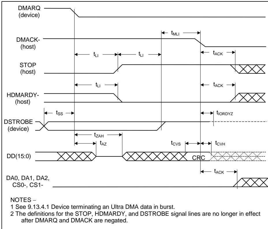
Figure 74 – Device terminating an Ultra DMA data-in burst
