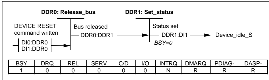
Figure 63 – Device DEVICE RESET command state diagram
