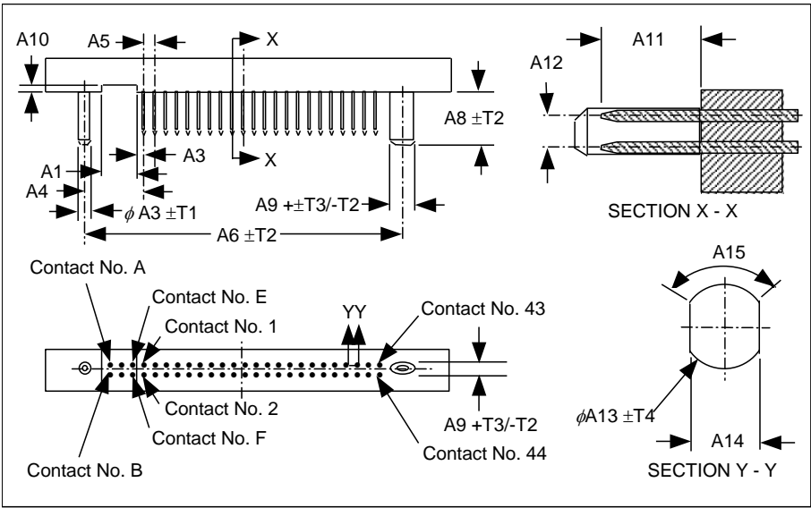
Figure 18 – 1.8 inch 3.3 V parallel host connector
