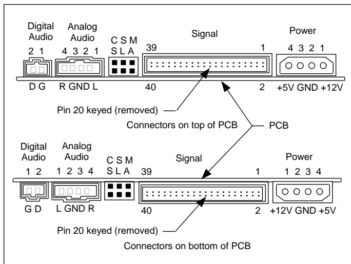
Figure 28 – 5.25 inch CD-ROM connector location
