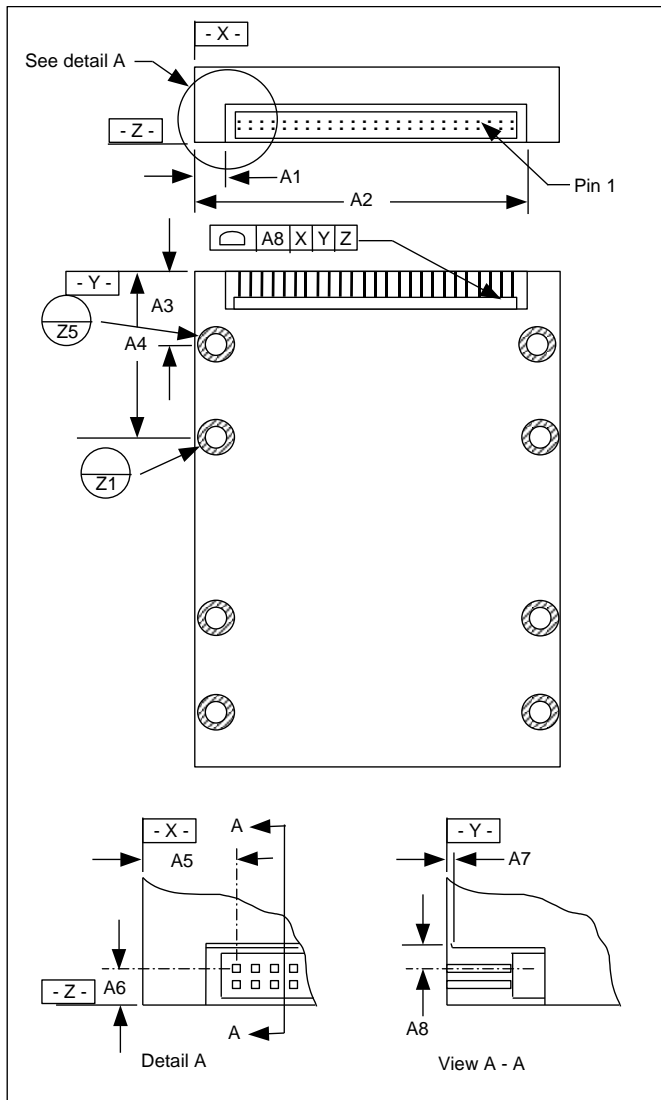
Figure 22 – 2.5" form factor connector location
