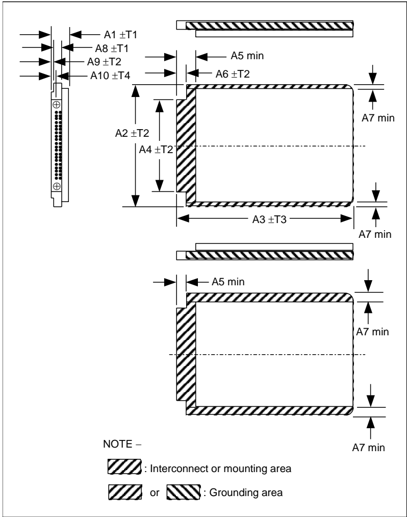
Figure 25 – 1.8 inch 3.3V parallel form factor
