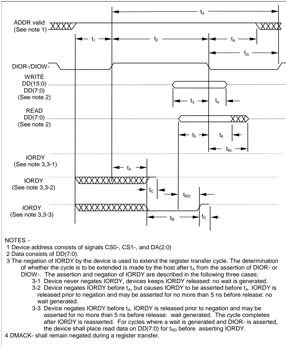
Figure 66 – PIO data transfer to/from device
