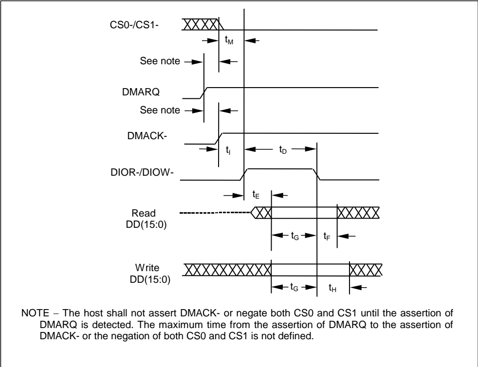
Figure 67 – Initiating a Multiword DMA data burst
