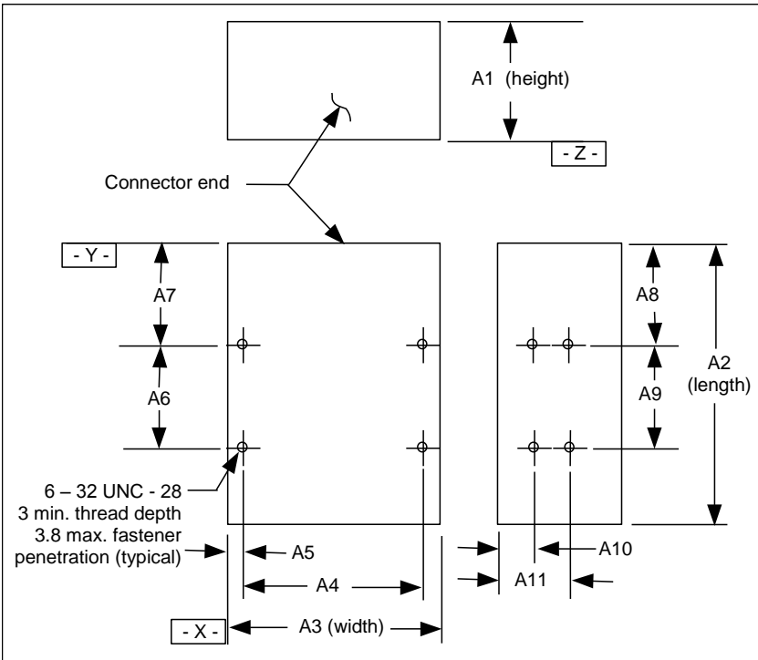
Figure 26 – 5.25 inch HDD form factor
