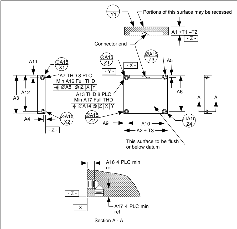
Figure 23 – 1.8 inch 5V parallel form factor
