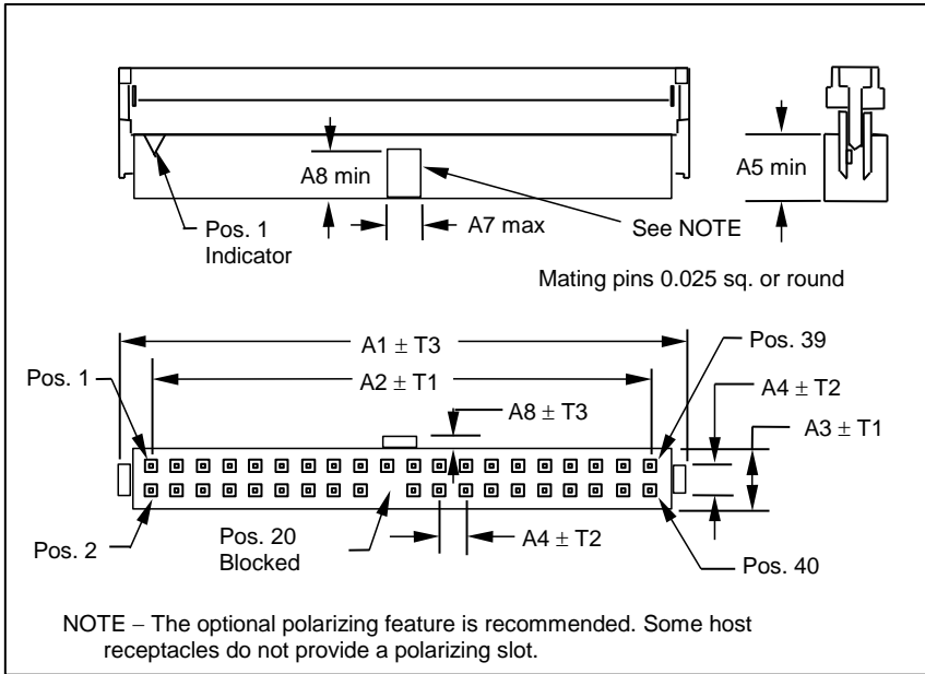
Figure 6 – 40-pin I/O cable connector
