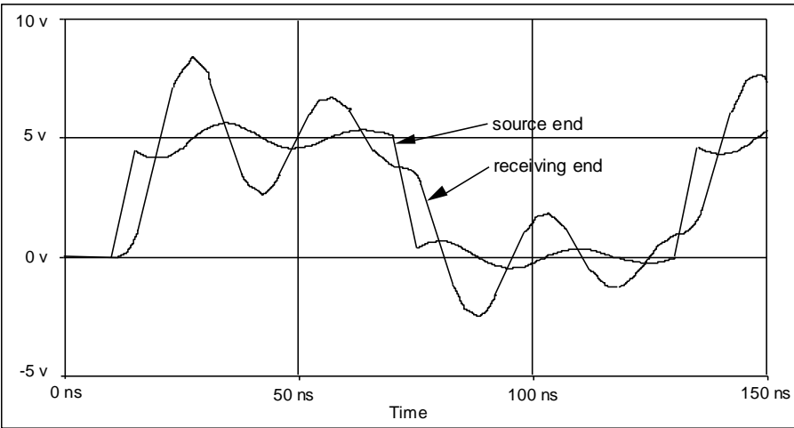
Figure 104 - Output of Simple RLC model: waveforms at source and receiving connectors
