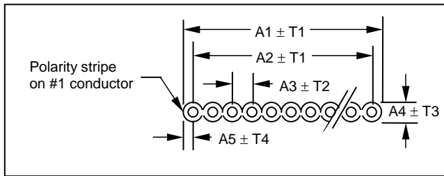
Figure 9 – 80-conductor ribbon cable
