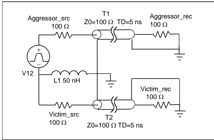
Figure 101 - Model of ground bounce in IC package
