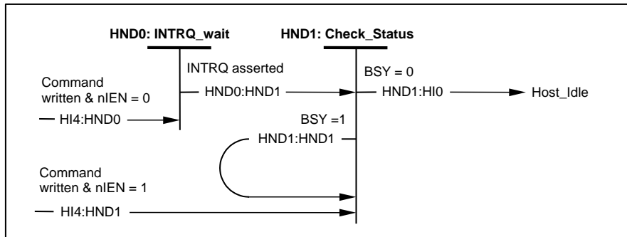
Figure 45 – Host Non-Data state diagram
