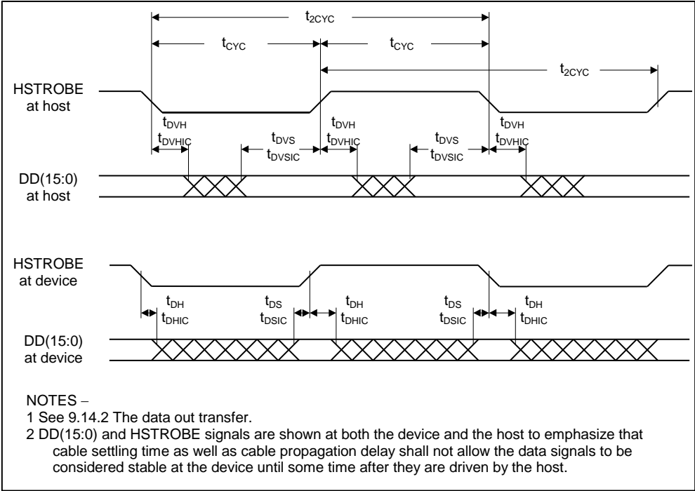
Figure 77 – Sustained Ultra DMA data-out burst
