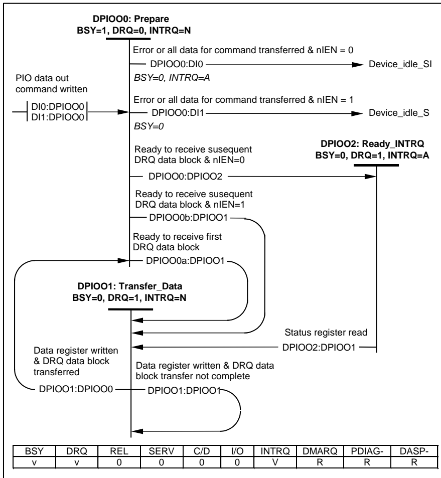
Figure 50 – Device PIO data-Out state diagram
