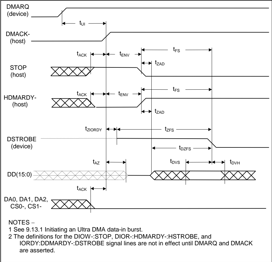
Figure 71 – Initiating an Ultra DMA data-in burst
