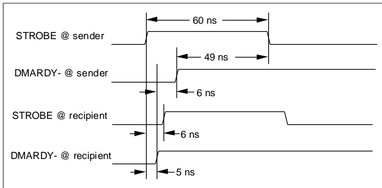
Figure 112 - STROBE and DMARDY- at sender and recipient
