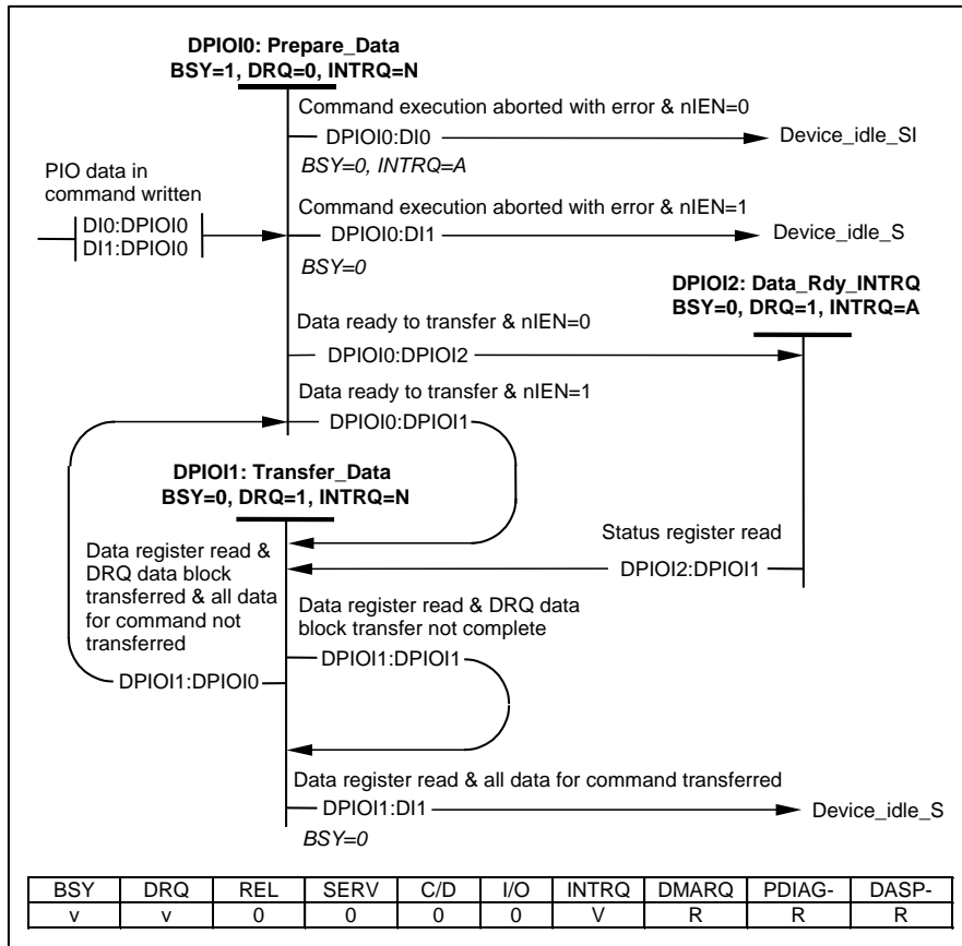
Figure 48 – Device PIO data-In state diagram
