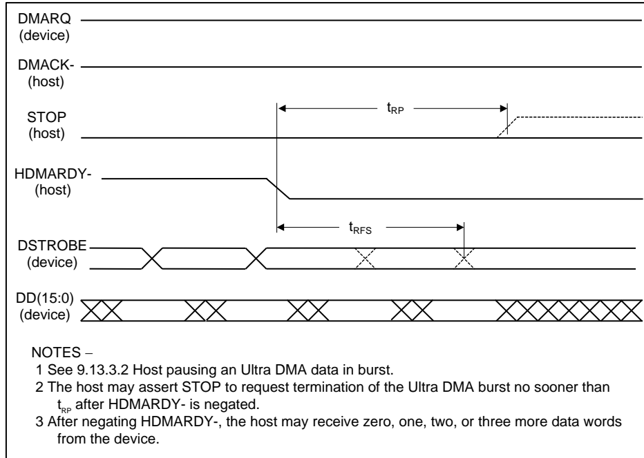
Figure 73 – Host pausing an Ultra DMA data-in burst
