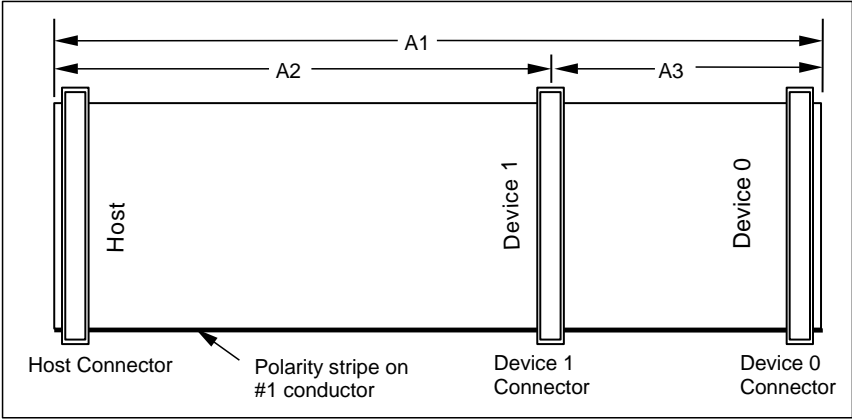
Figure 10 – 80-conductor cable configuration
