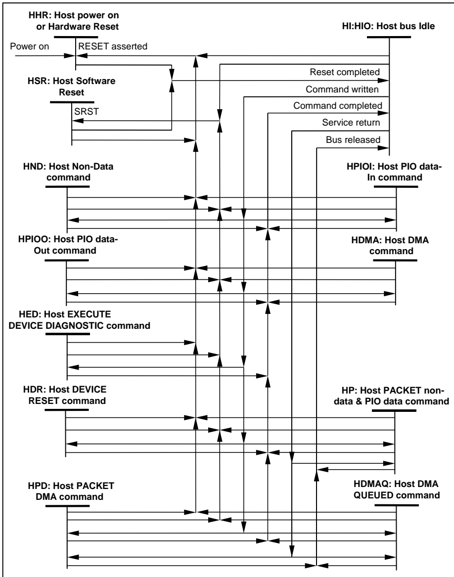
Figure 34 – Overall host protocol state sequence
