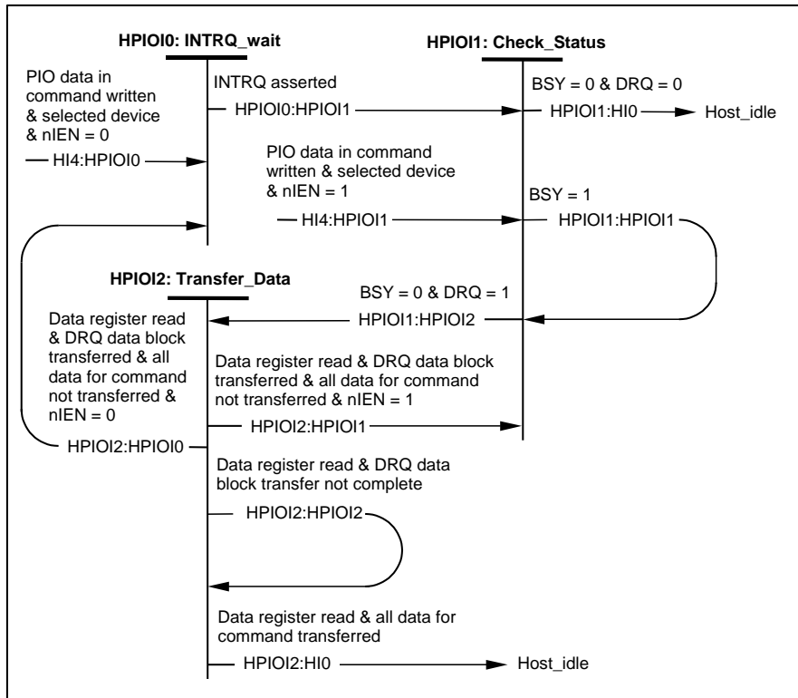
Figure 47 – Host PIO data-In state diagram
