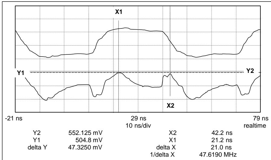
Figure 90 - Reverse crosstalk waveform from reflected edge
