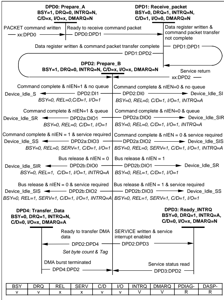
Figure 56 – Device PACKET DMA command state diagram
