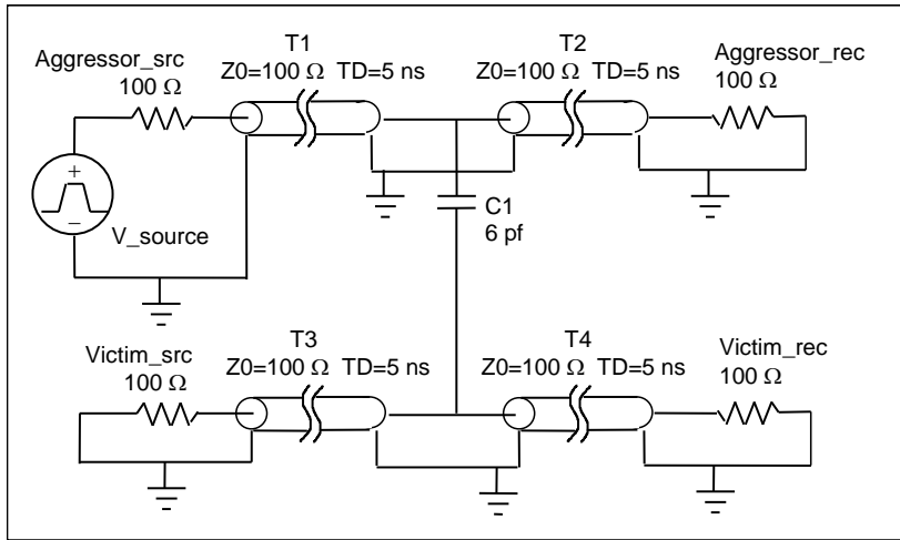
Figure 91 - Model of capacitive coupling
