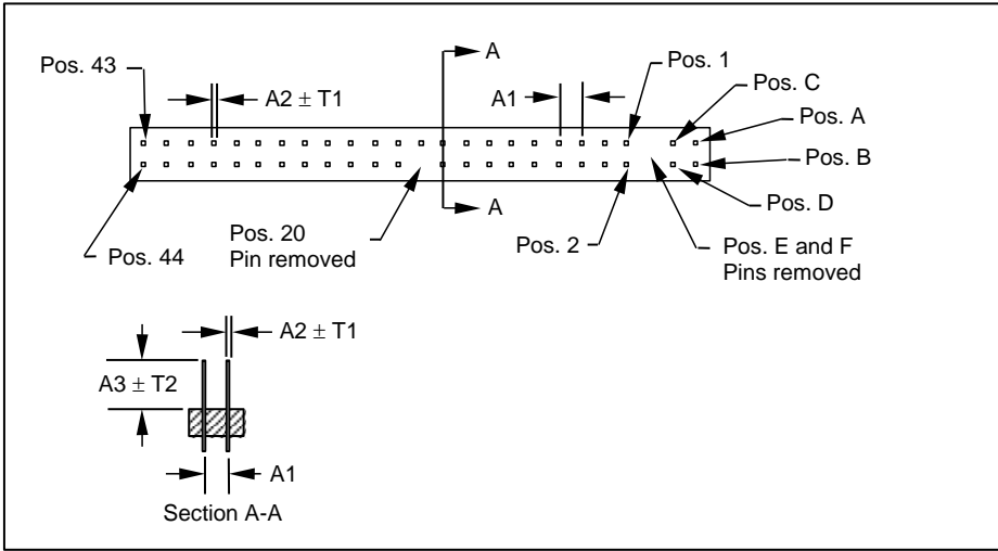
Figure 16 – 50-pin 2.5 inch form factor style connector
