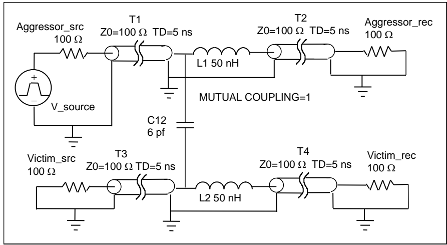
Figure 95 - Model of capacitive and inductive coupling
