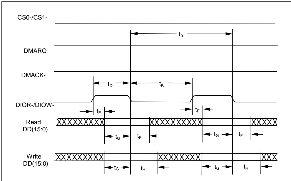
Figure 68 - Sustaining a Multiword DMA data burst
