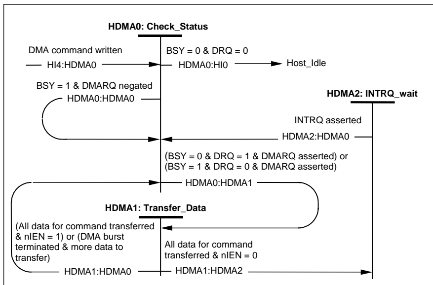
Figure 51 – Host DMA state diagram
