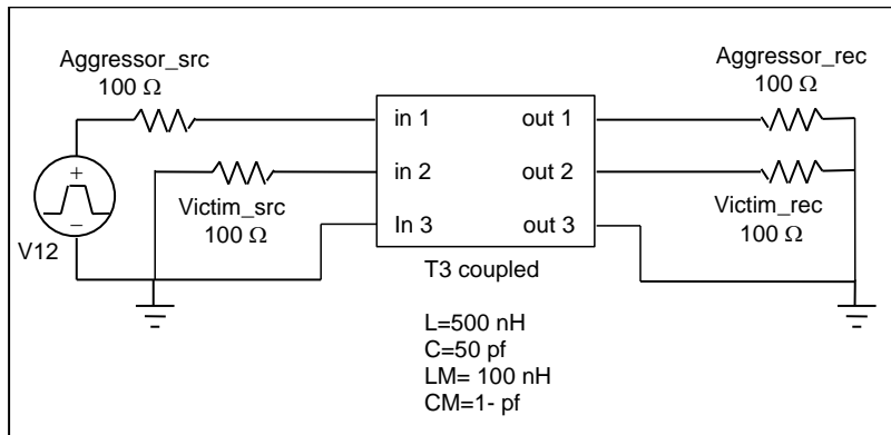
Figure 97 - Model of distributed coupling
