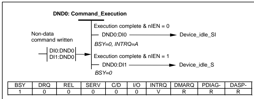
Figure 46 – Device Non-Data state diagram
