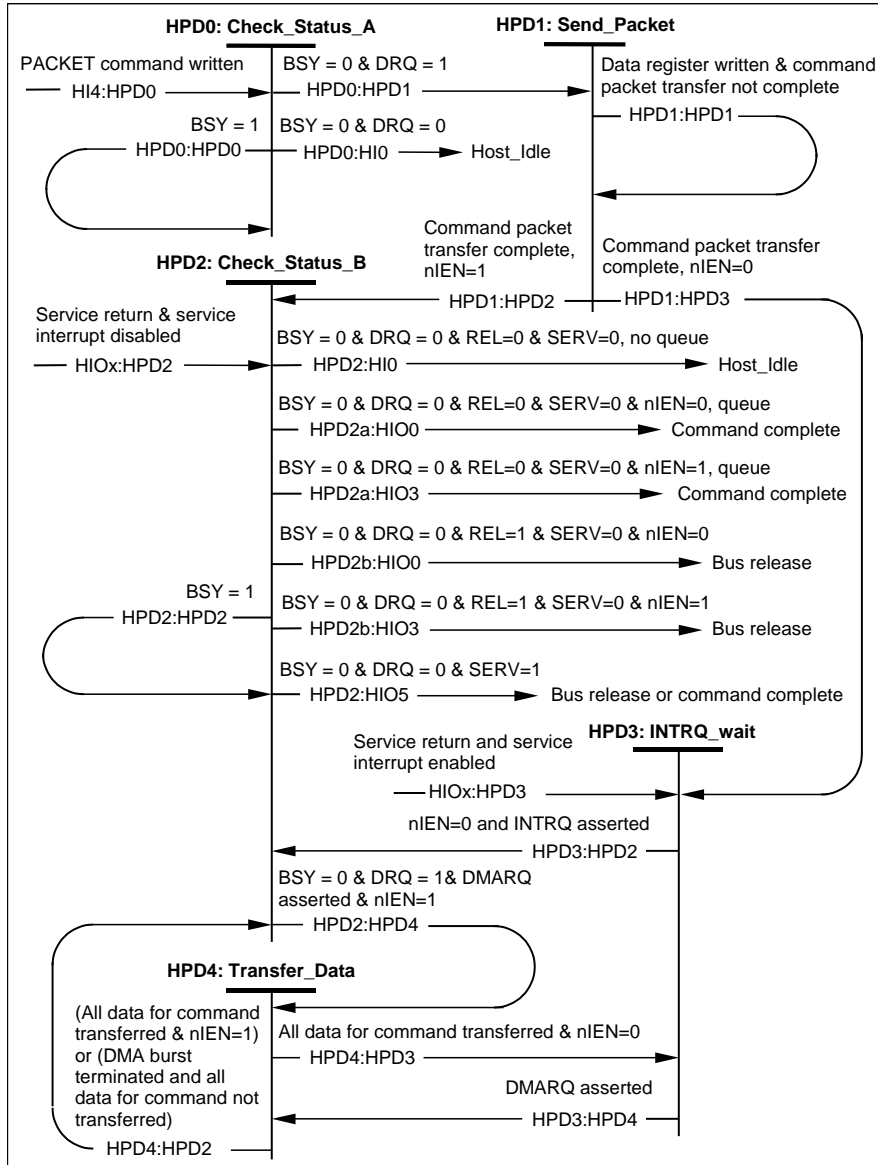
Figure 55 – Host PACKET DMA command state diagram
