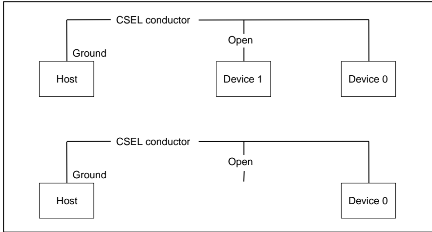
Figure 30 – Alternate cable select example
