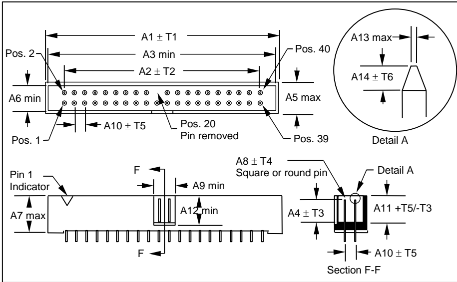
Figure 5 – Host or device 40-pin I/O header
