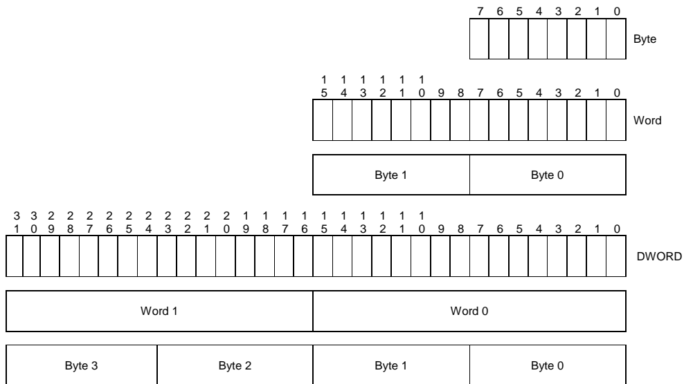
Figure 3 - Byte, word and DWORD relationships
