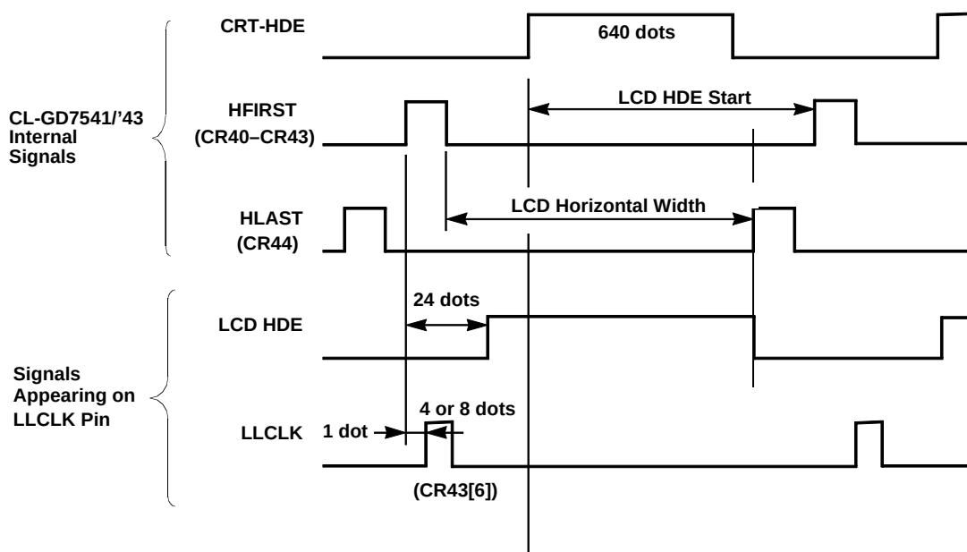
Figure 12-4. Horizontal Position for STN LCD Displaying 640 \times 480 Picture
