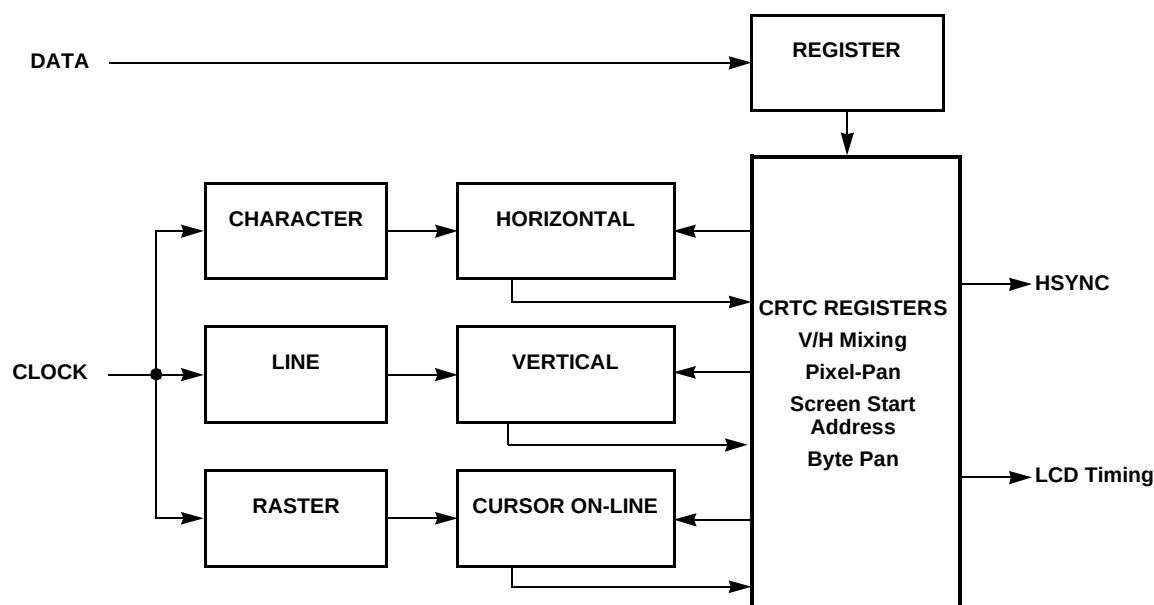
Figure 3-5. CRT Controller Functional Block Diagram
