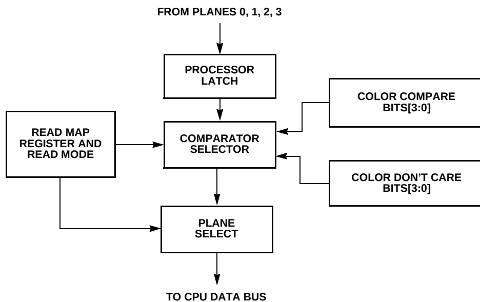
Figure 3-3. Graphics Controller Read Operation
