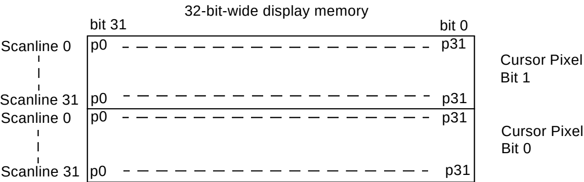
Figure B-1. Mapping of 32 × 32 Hardware Cursor
