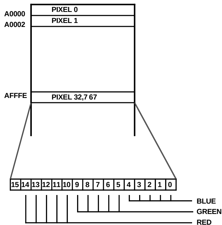
Figure K-3. 32,768 Color (15-Bit) Packed-Pixel Mode
