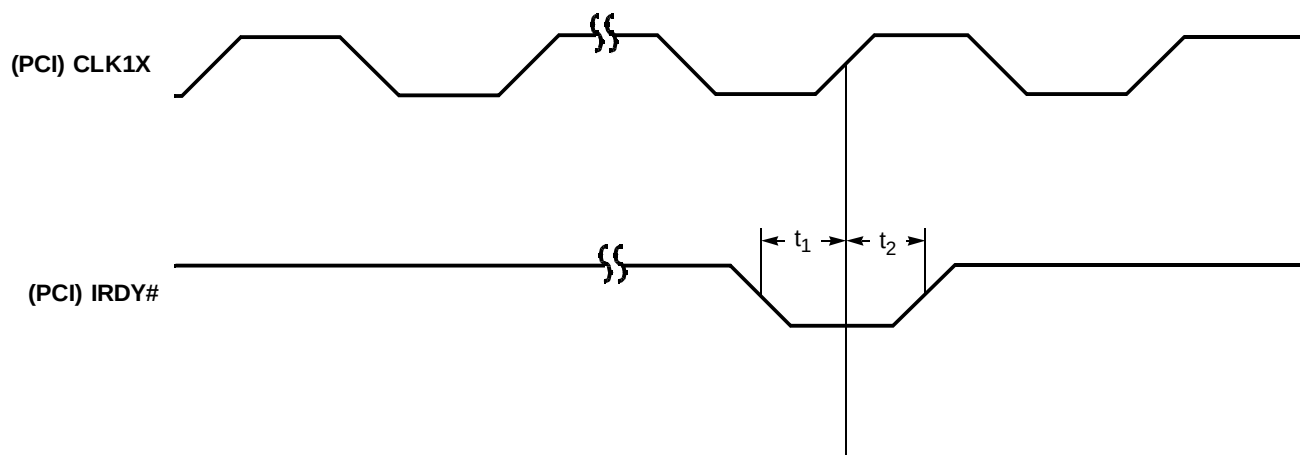
Figure 13-10. PCI Bus — Read Data / IRDY# Timing
