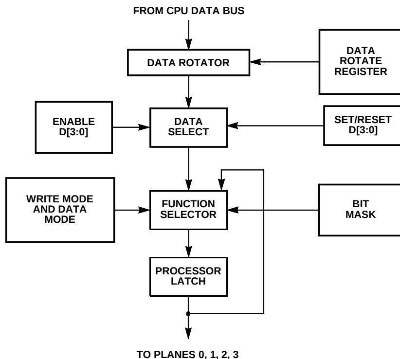
Figure 3-2. Graphics Controller Write Operation
