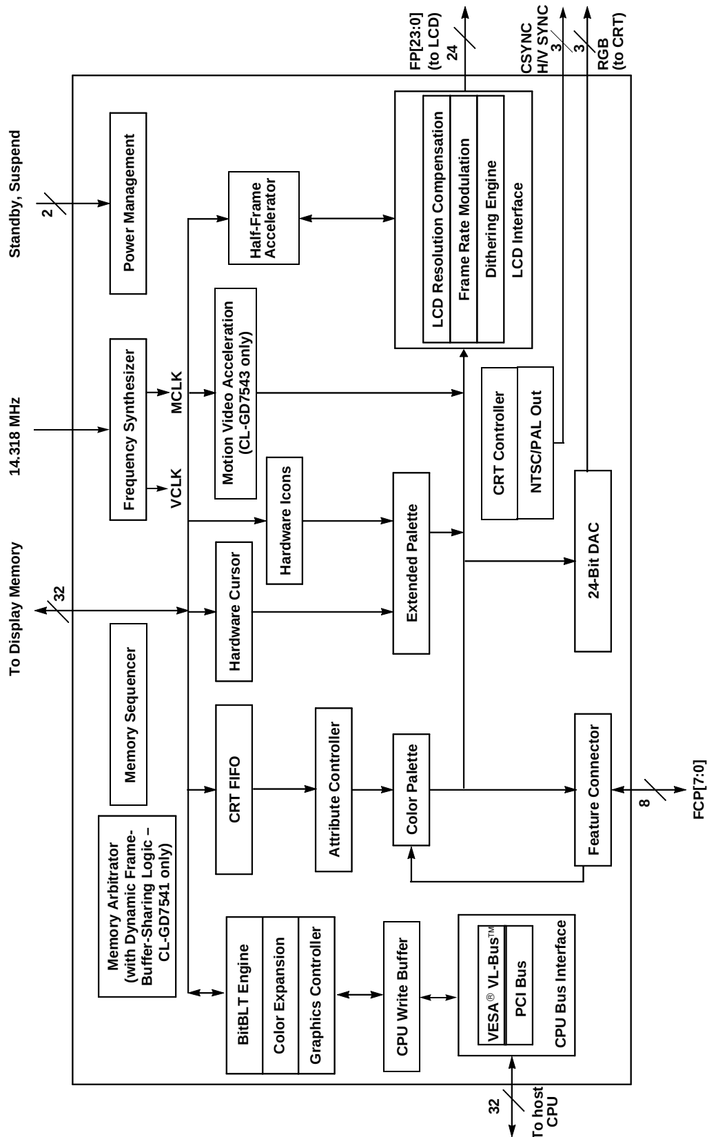
Figure 3-1. CL-GD7541/GD7543 Block Diagram
