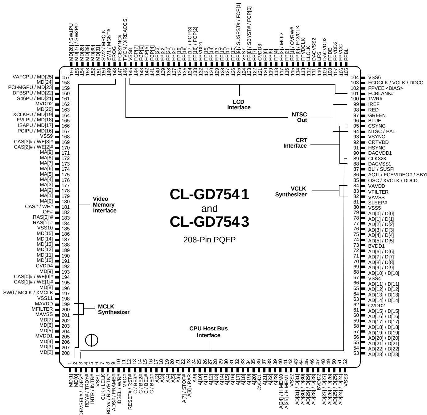
Figure 1-1. Pin Diagram
