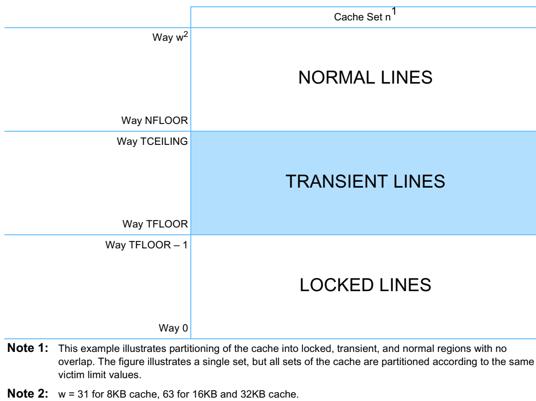
Figure 4-3. Cache Locking and Transient Mechanism (Example 1) 1
