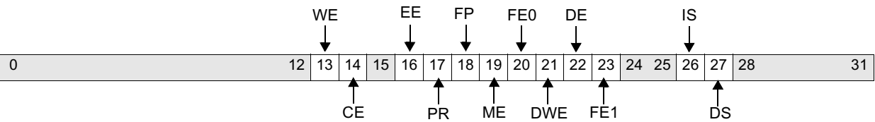
Figure 6-5. Critical Save/Restore Register 1 (CSRR1)
