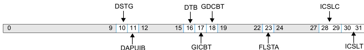
Figure 4-5. Core Configuration Register 0 (CCR0)
