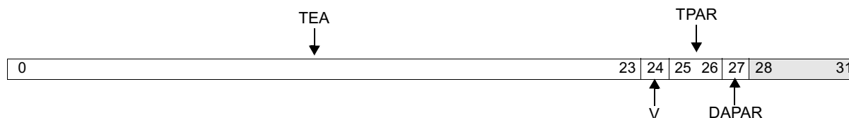
Figure 10-25. Instruction Cache Debug Tag Register High (ICDBTRH)
