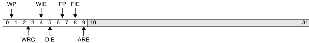
Figure 10-44. Timer Control Register (TCR)
