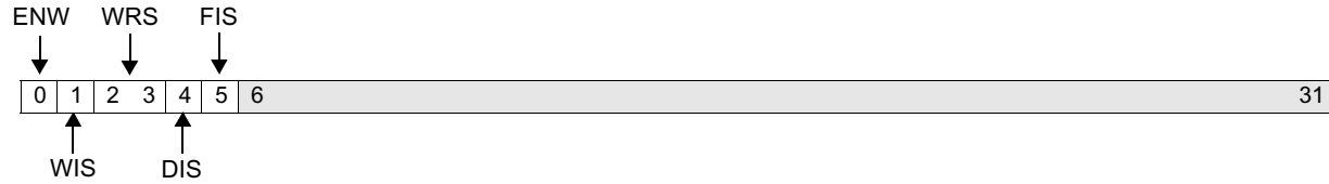
Figure 10-45. Timer Status Register (TSR)
