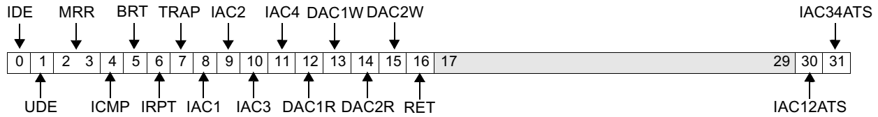
Figure 10-11. Debug Status Register (DBSR)
