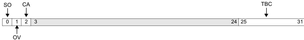
Figure 10-47. Integer Exception Register (XER)
