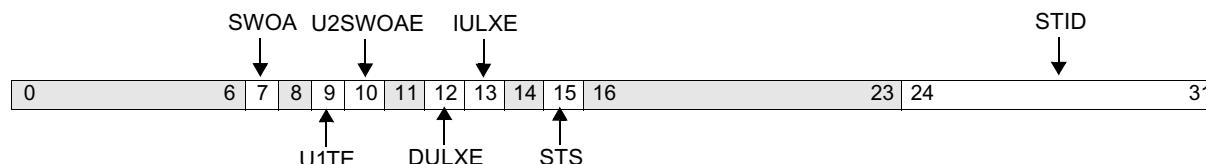
Figure 10-33. Memory Management Unit Control Register (MMUCR)
