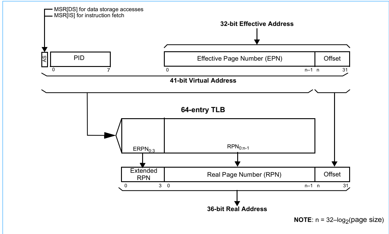
Figure 5-2. Effective-to-Real Address Translation Flow
