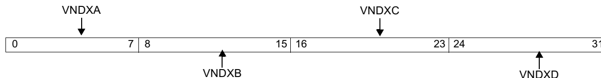
Figure 10-18. Data Cache Transient Victim Registers (DTV0–DTV3)
