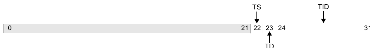
Figure 4-8. Instruction Cache Debug Tag Register Low (ICDBTRL)
