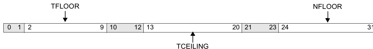
Figure 10-20. Data Cache Victim Limit (DVLIM)
