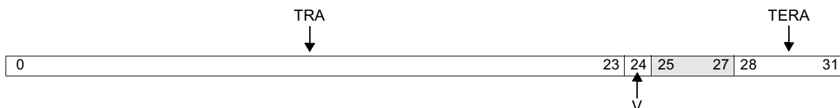
Figure 4-9. Data Cache Debug Tag Register High (DCDBTRH)
