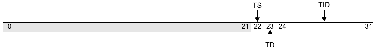
Figure 10-26. Instruction Cache Debug Tag Register Low (ICDBTRL)
