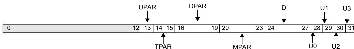
Figure 4-10. Data Cache Debug Tag Register Low (DCDBTRL)
