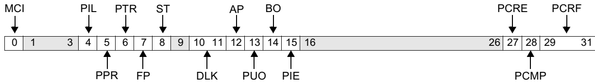
Figure 10-21. Exception Syndrome Register (ESR)
