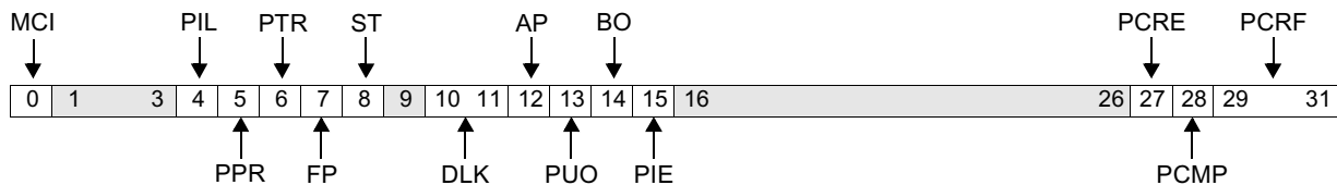
Figure 6-9. Exception Syndrome Register (ESR)
