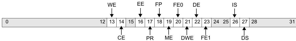
Figure 10-34. Machine State Register (MSR)
