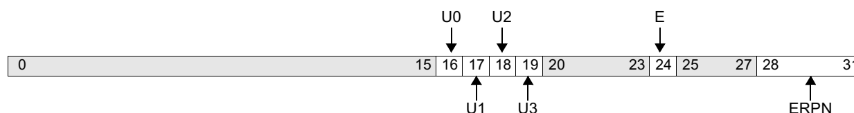
Figure 2-12. Reset Configuration
