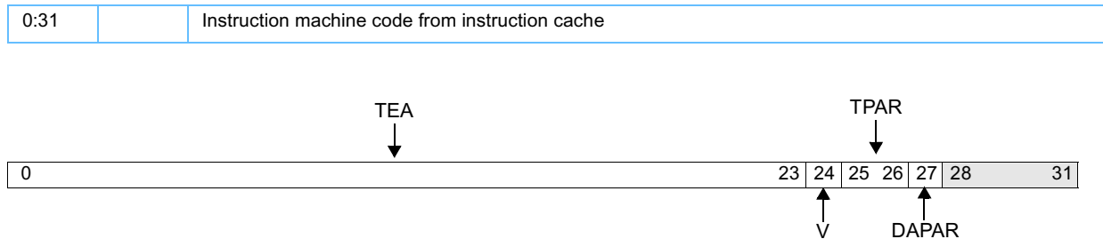
Figure 4-6. Instruction Cache Debug Data Register (ICDBDR)
