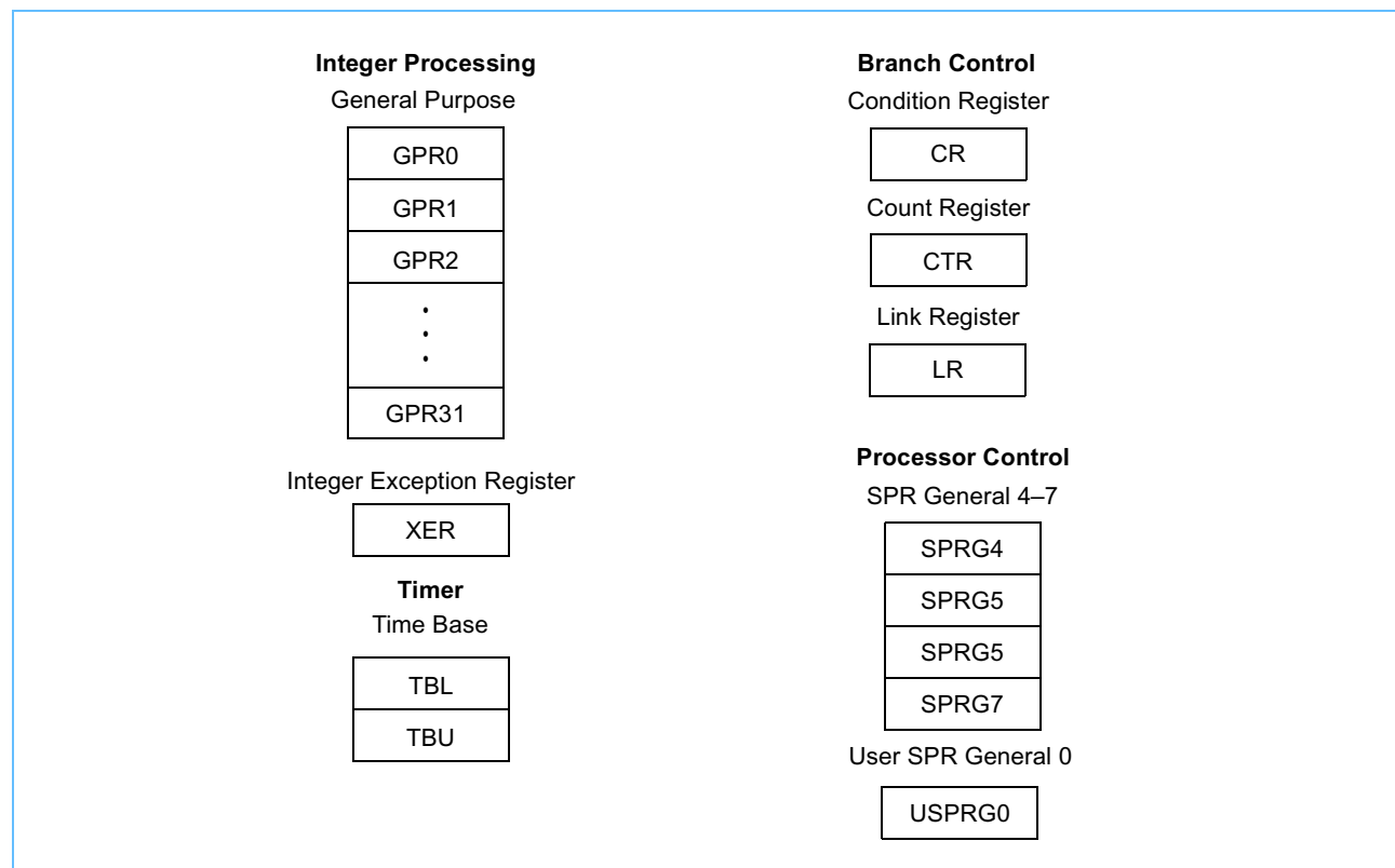
Figure 2-1. User Programming Model Registers
