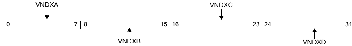
Figure 10-27. Instruction Cache Normal Victim Registers (INV0–INV3)
