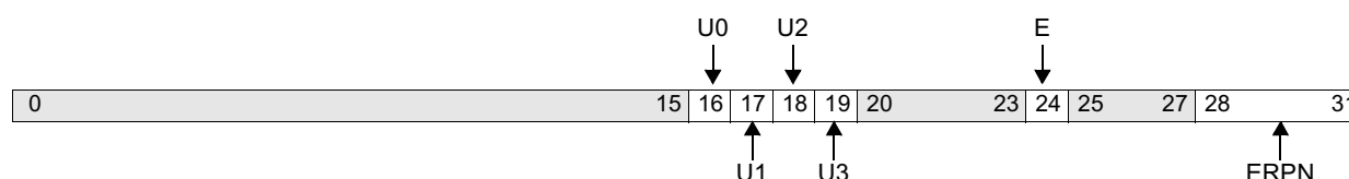
Figure 10-38. Reset Configuration
