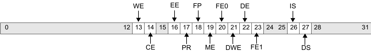
Figure 10-4. Critical Save/Restore Register 1 (CSRR1)
