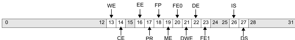
Figure 6-1. Machine State Register (MSR)
