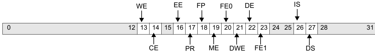
Figure 10-41. Save/Restore Register 1 (SRR1)
