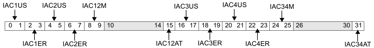
Figure 10-8. Debug Control Register 1 (DBCR1)
