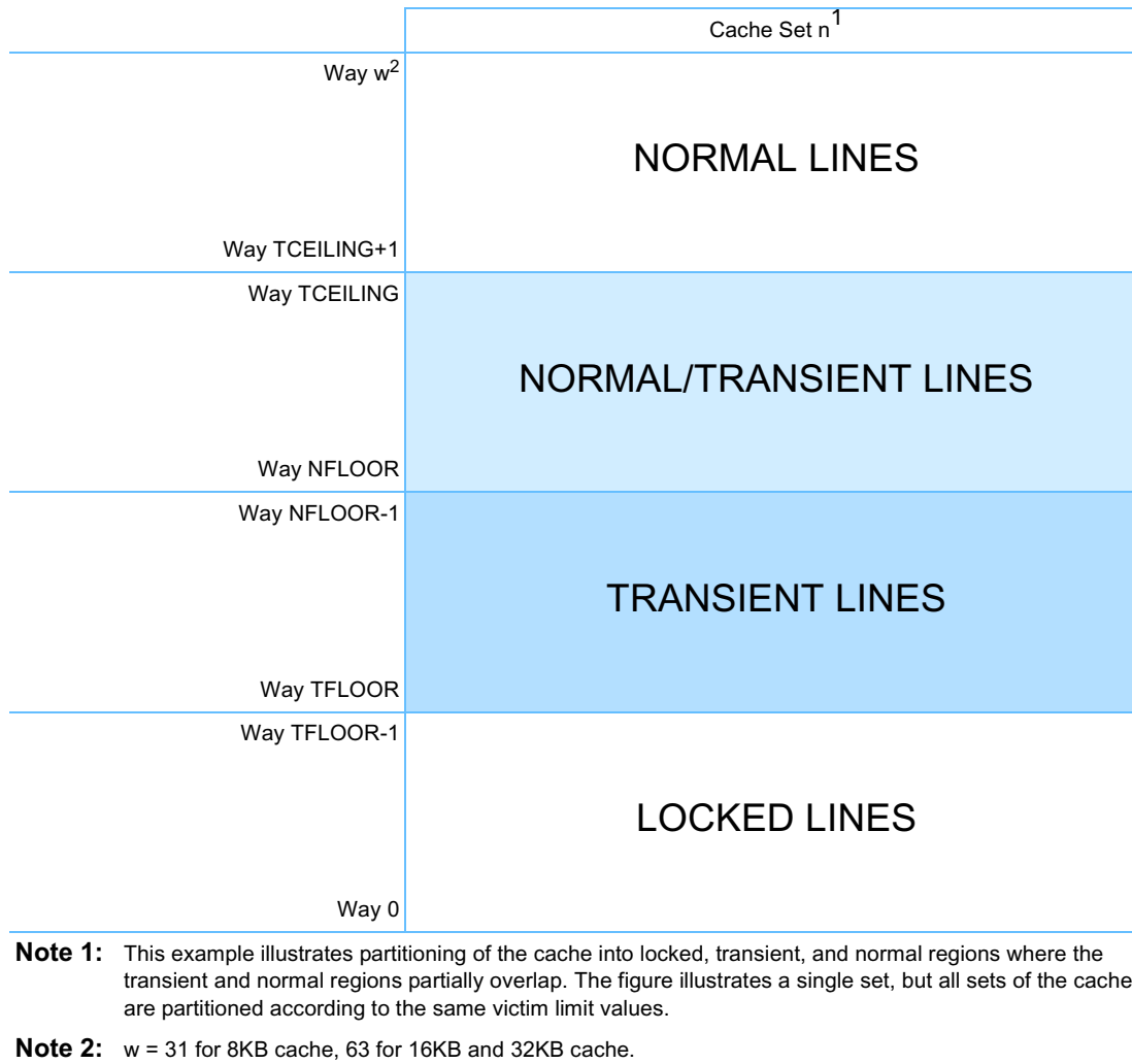
Figure 4-4. Cache Locking and Transient Mechanism (Example 2)
