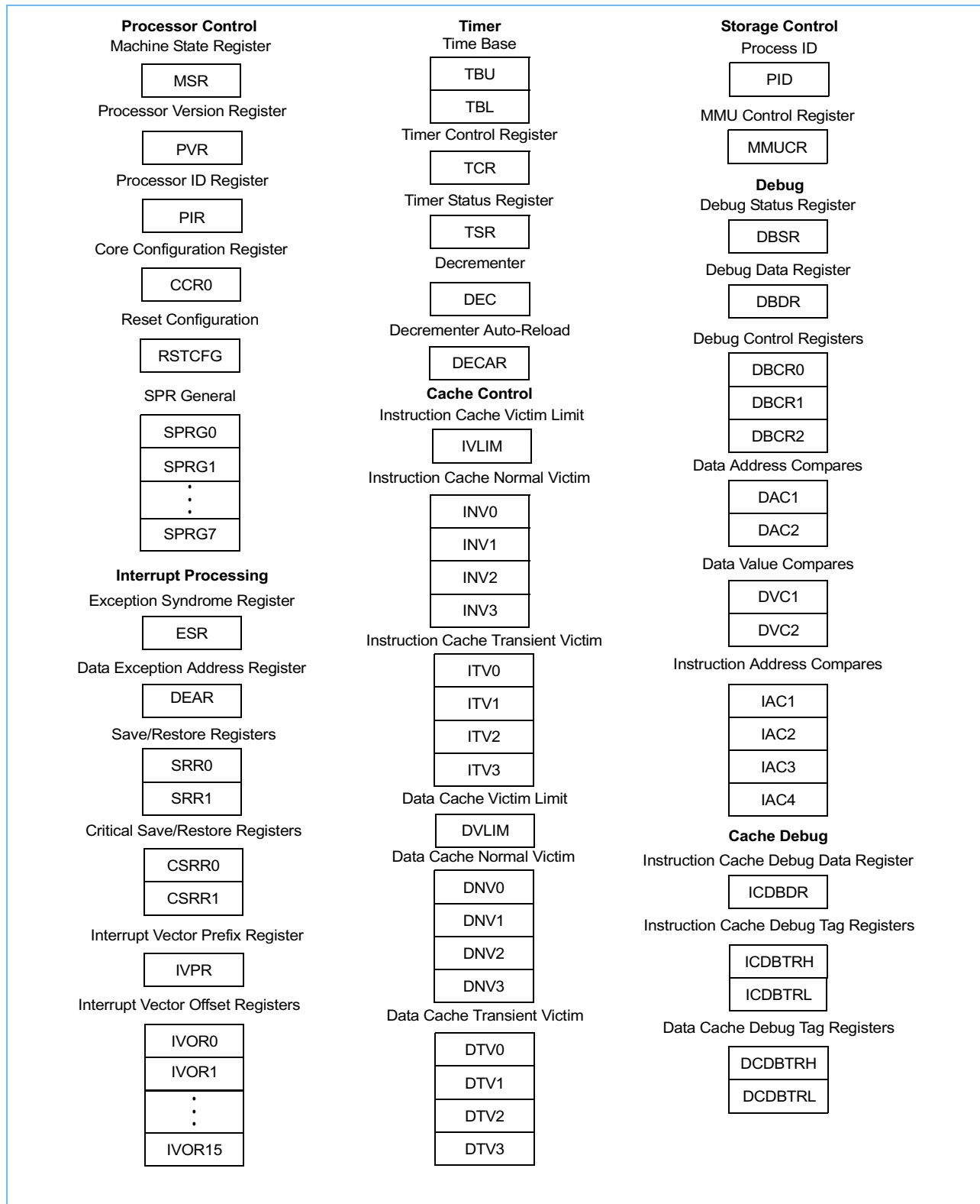
Figure 2-2. Supervisor Programming Model Registers
