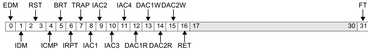
Figure 10-7. Debug Control Register 0 (DBCR0)
