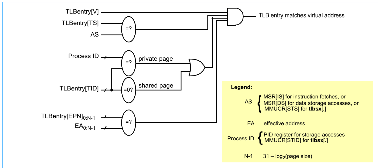
Figure 5-1. Virtual Address to TLB Entry Match Process
