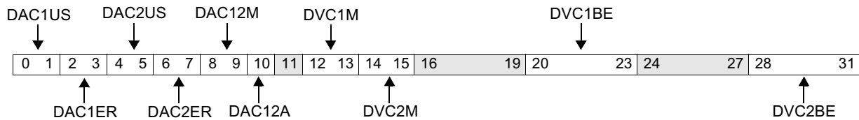
Figure 10-9. Debug Control Register 2 (DBCR2)
