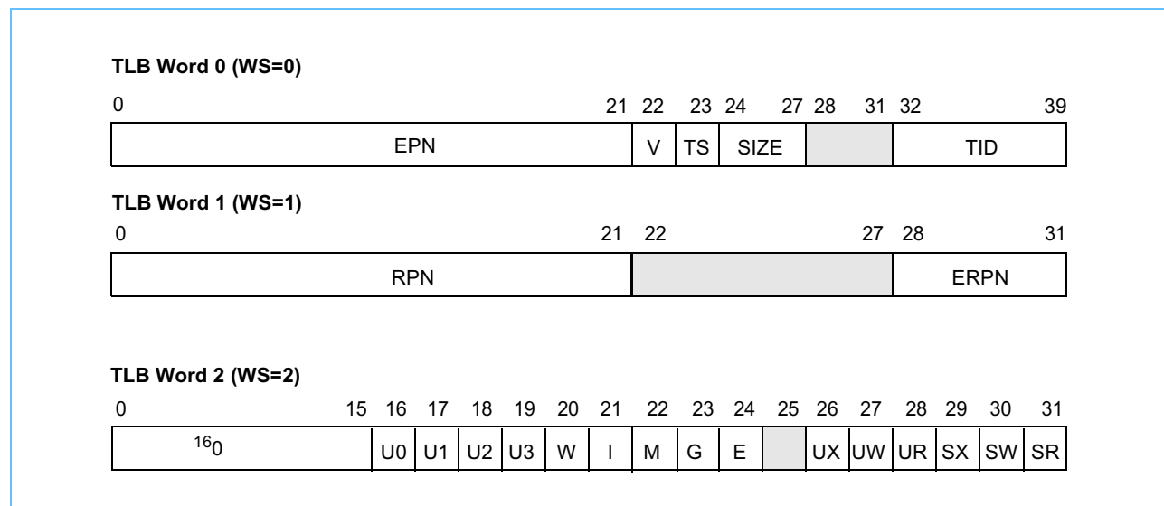
Figure 5-5. TLB Entry Word Definitions
