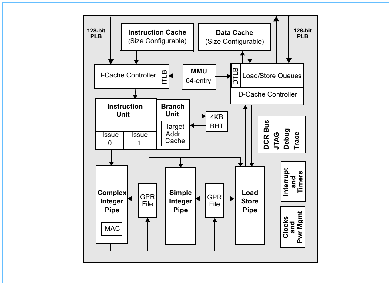
Figure 1-1. PPC440x4 Core Block Diagram
