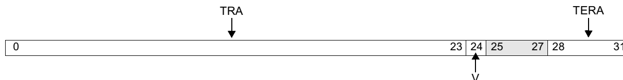
Figure 10-12. Data Cache Debug Tag Register High (DCDBTRH)
