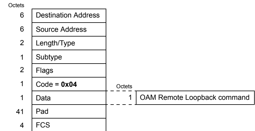
Figure 57–14—Loopback Control OAMPDU frame structure
