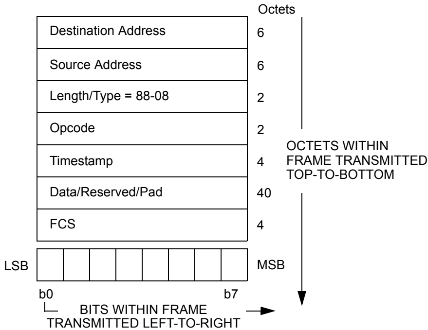
Figure 64–30—Generic MPCPDU
