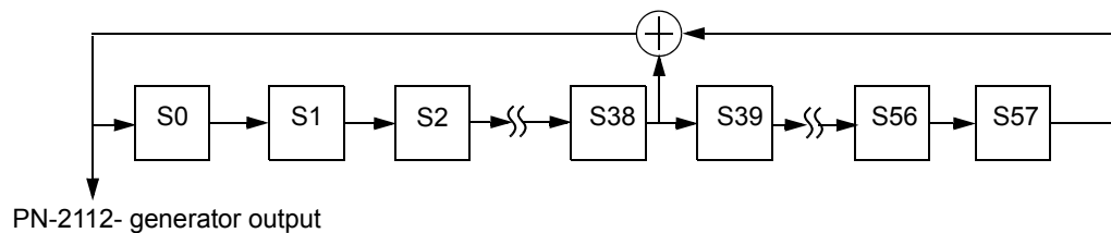
Figure 74-5—PN-2112 generator
