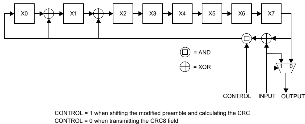
Figure 65–2—CRC8 field generation
