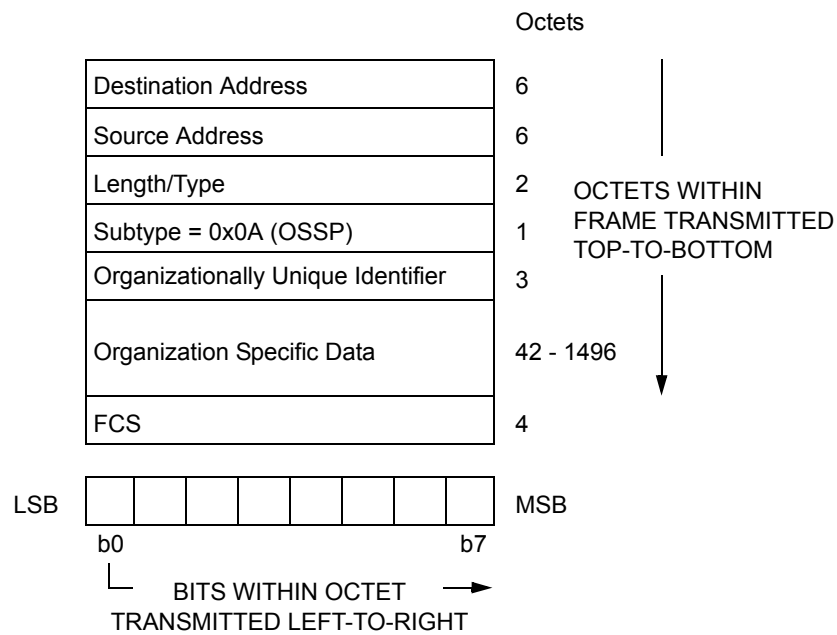
Figure 57B-1—OSSPDU structure
