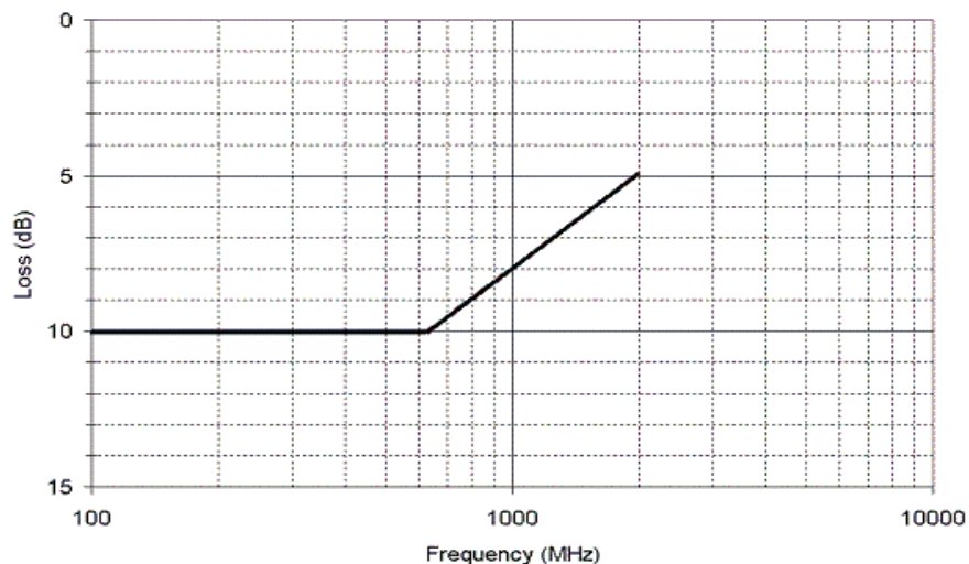
Figure 71-4—Minimum differential output return loss
