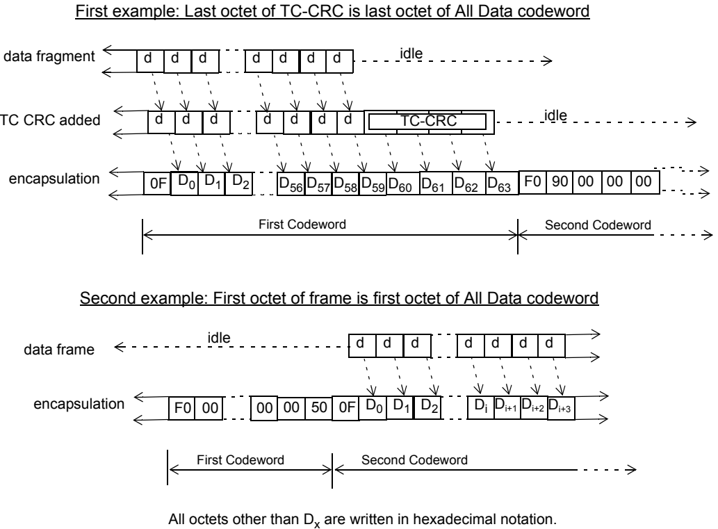
Figure 61–15—TC Encapsulation examples
