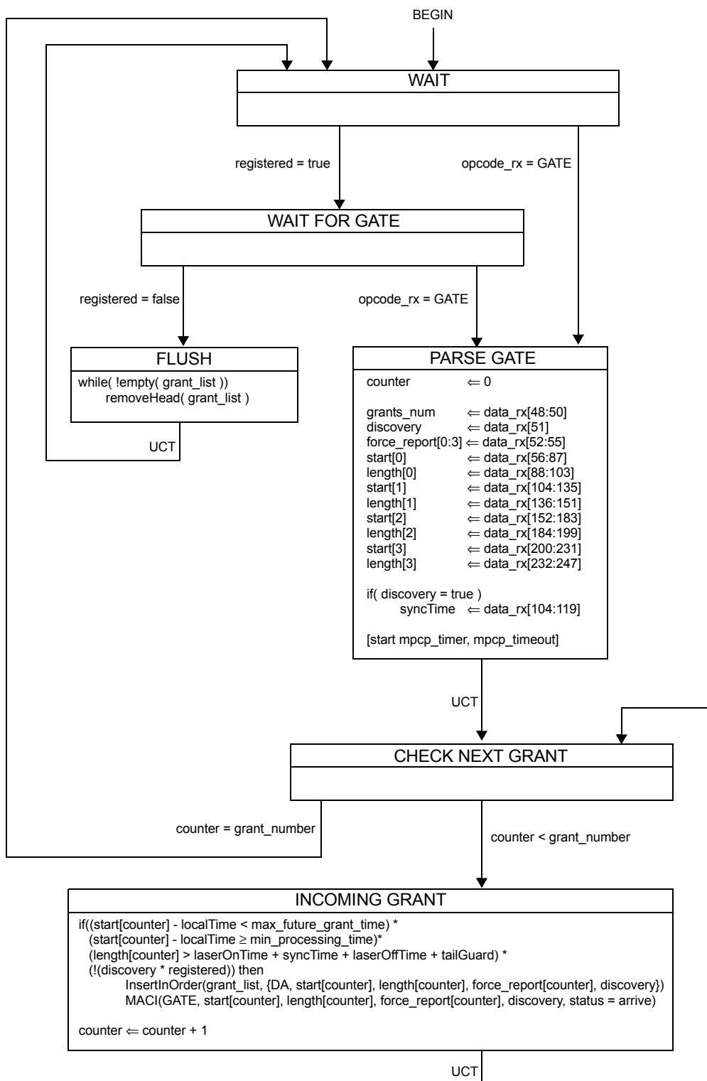
Figure 64-28—Gate Processing ONU Programing State Diagram
