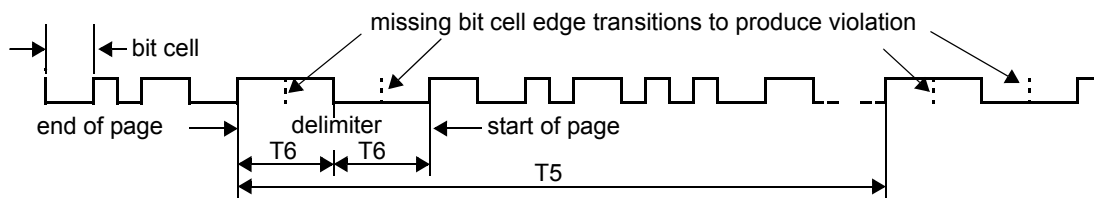
Figure 73–5—Manchester violation
