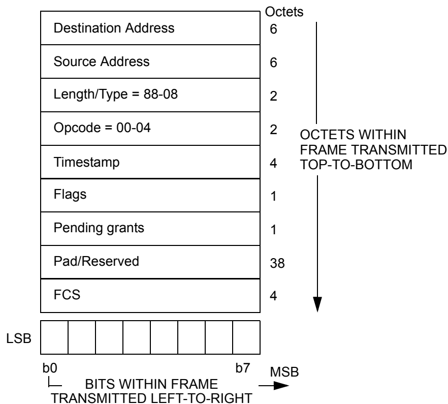
Figure 64–33—REGISTER_REQ MPCPDU
