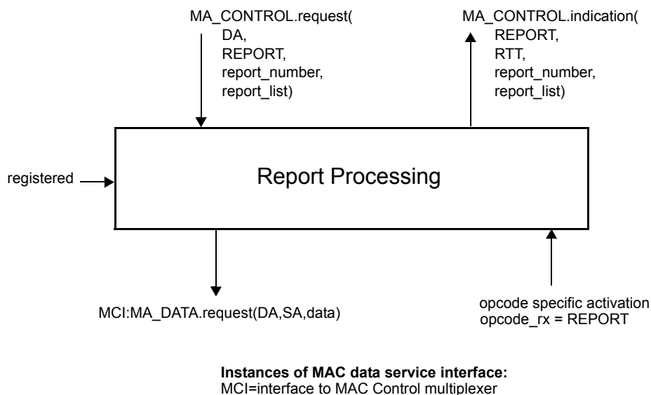
Figure 64–23—Report Processing service interfaces
