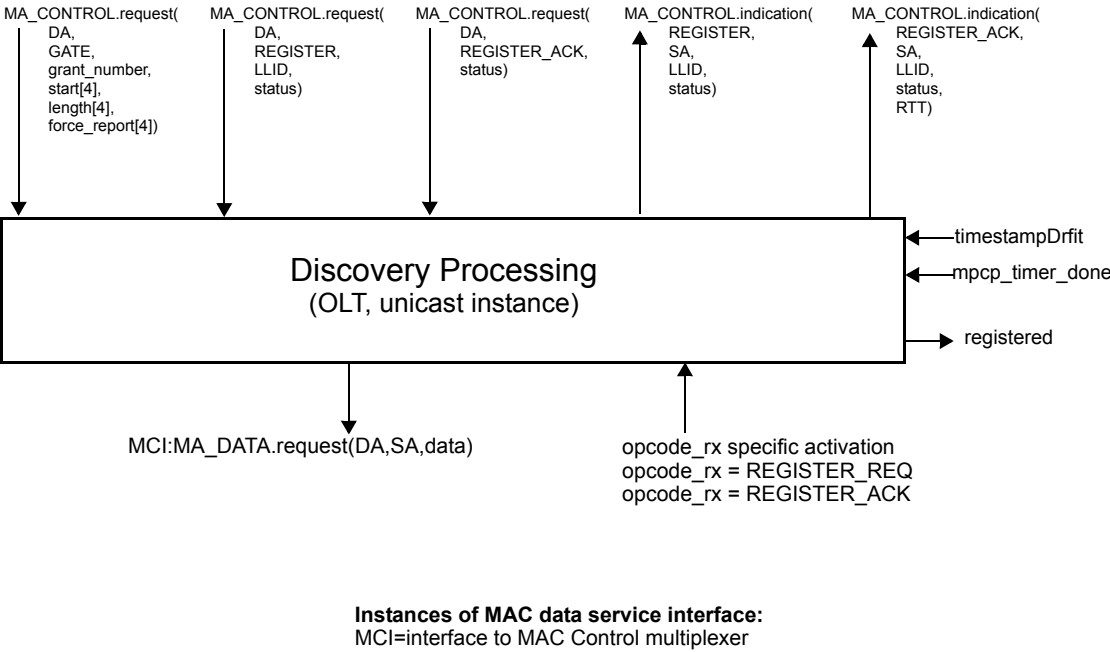
Figure 64–16—Discovery Processing service interfaces (OLT, unicasting instance)
