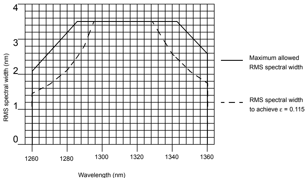
Figure 59-3—1000BASE-LX-10 Transmitter spectral limits
