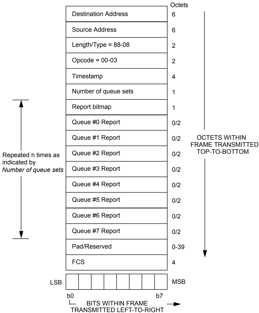
Figure 64–32—REPORT MPCPDU
