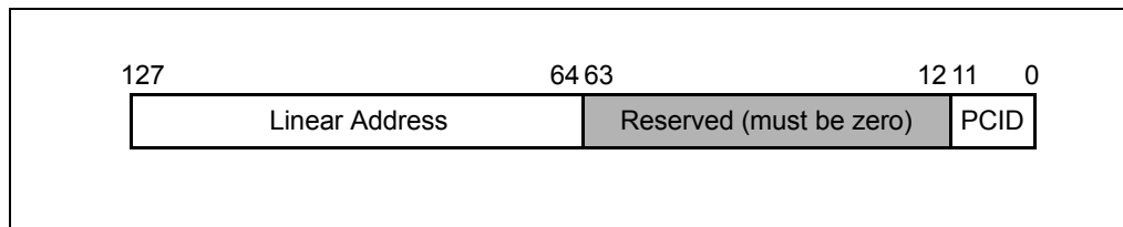
Figure 3-23. INVPCID Descriptor
