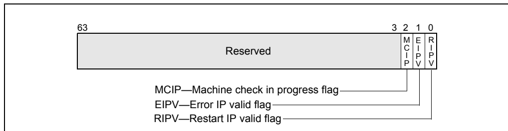
Figure 15-3. IA32_MCG_STATUS Register
