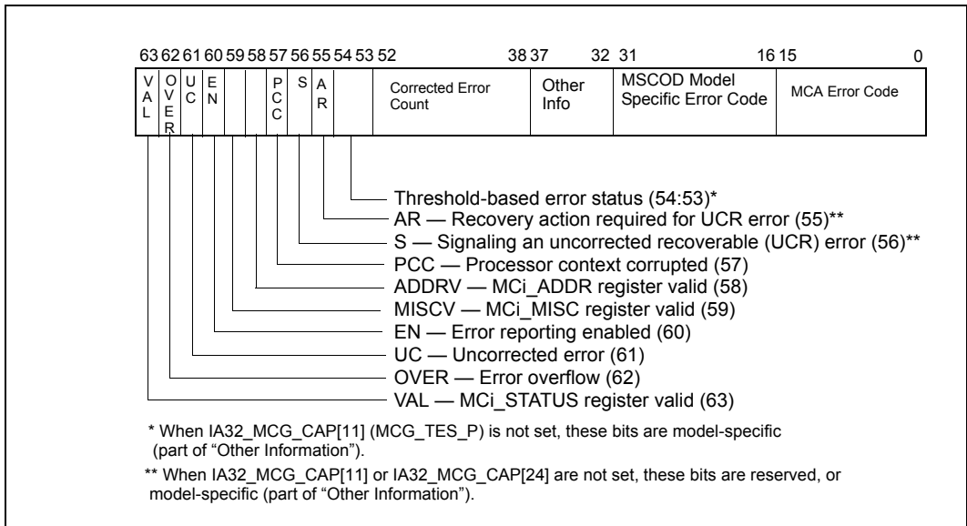
Figure 15-5. IA32_MCi_STATUS Register
