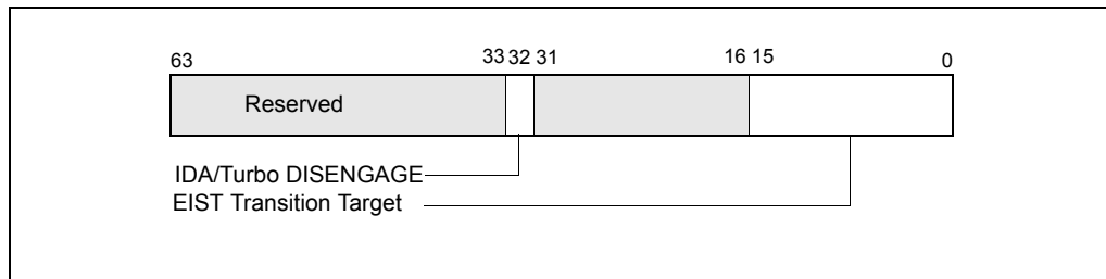
Figure 14-2. IA32_PERF_CTL Register
