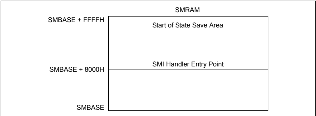
Figure 33-1. SMRAM Usage
