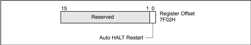
Figure 33-3. Auto HALT Restart Field
