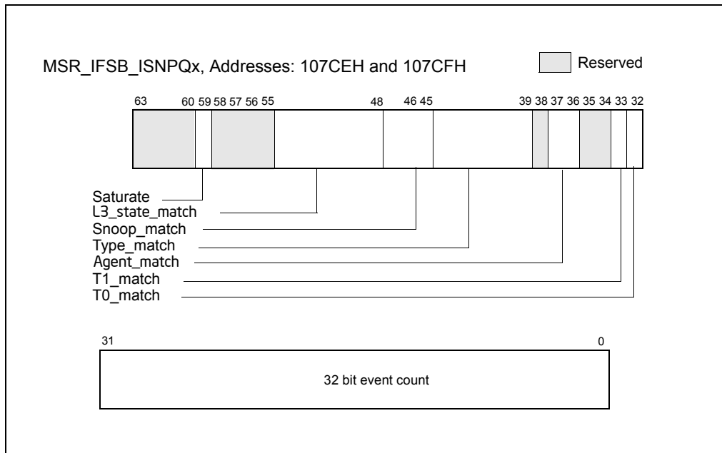
Figure 18-42. MSR_IFSB_ISNPQx, Addresses: 107CEH and 107CFH
