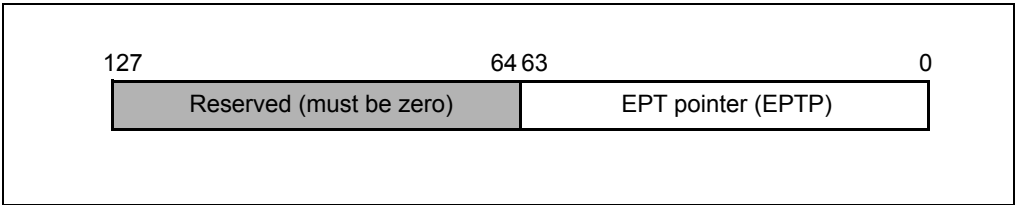
Figure 29-1. INVEPT Descriptor
