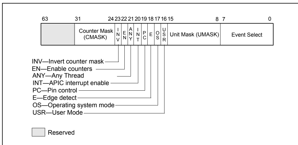
Figure 18-6. Layout of IA32_PERFEVTSELx MSRs Supporting Architectural Performance Monitoring Version 3
