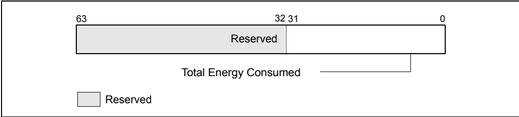
Figure 14-18. MSR_PKG_ENERGY_STATUS MSR
