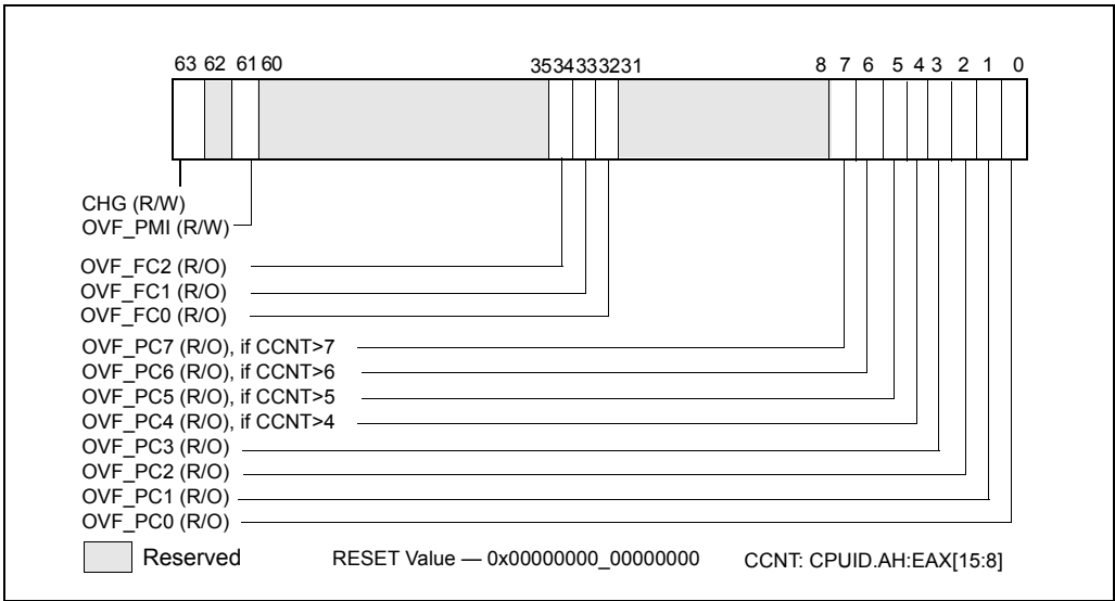
Figure 18-13. IA32_PERF_GLOBAL_STATUS MSR
