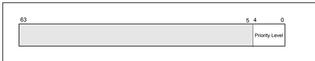
Figure 14-23. MSR_PP0_POLICY/MSR_PP1_POLICY Register
