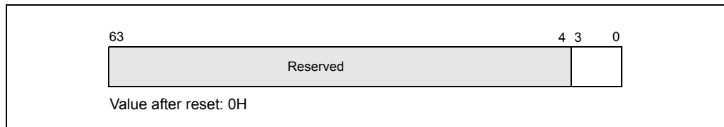
Figure 10-22. CR8 Register
