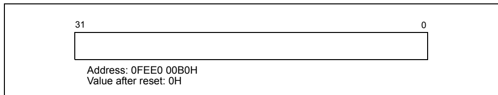
Figure 10-21. EOI Register
