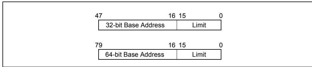
Figure 3-11. Pseudo-Descrptor Formats
