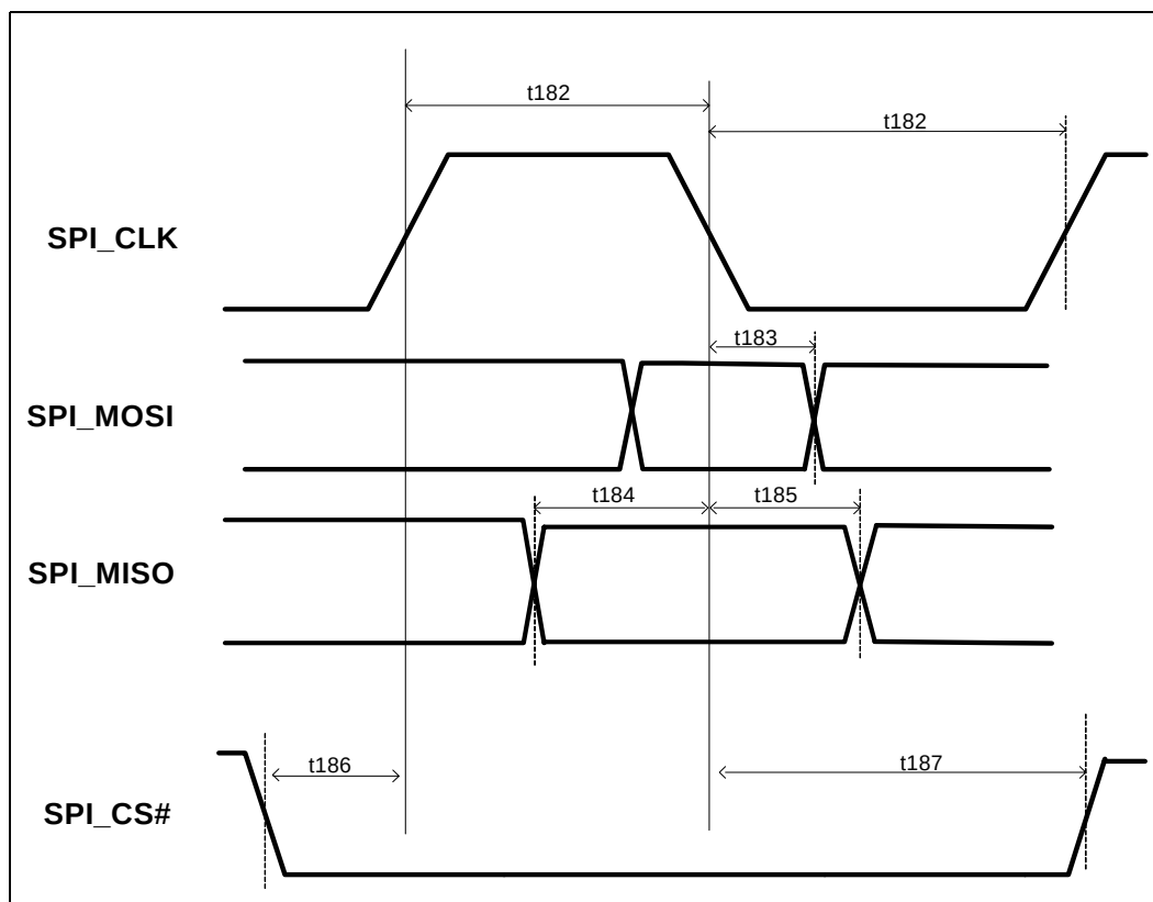
Figure 23-32. SPI Timings
