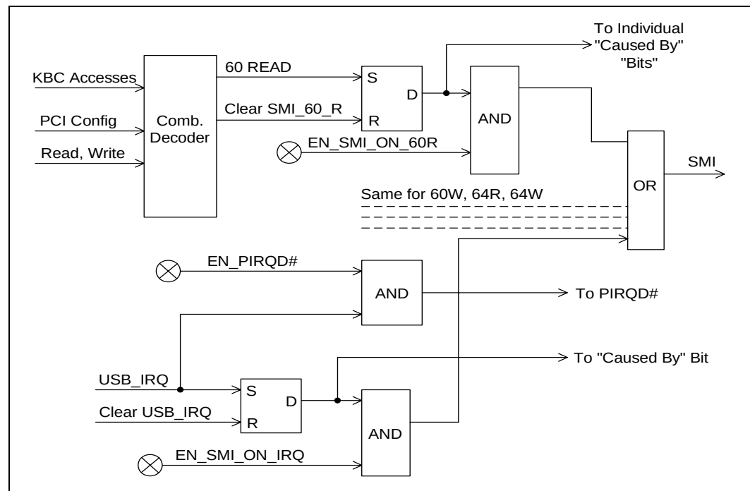
Figure 5-10. USB Legacy Keyboard Flow Diagram
