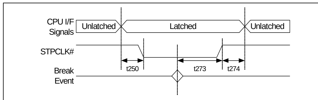
Figure 23-27. C0 to C2 to C0 Timings (Mobile Only)
