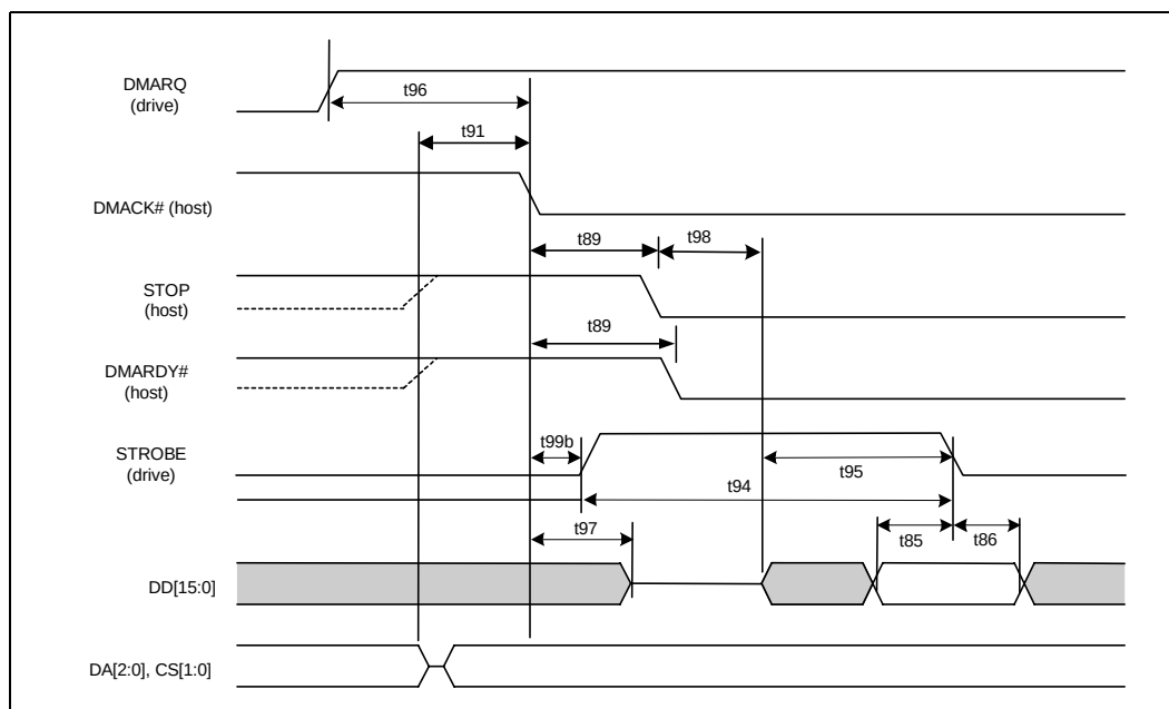
Figure 23-10. Ultra ATA Mode (Sustained Burst)
