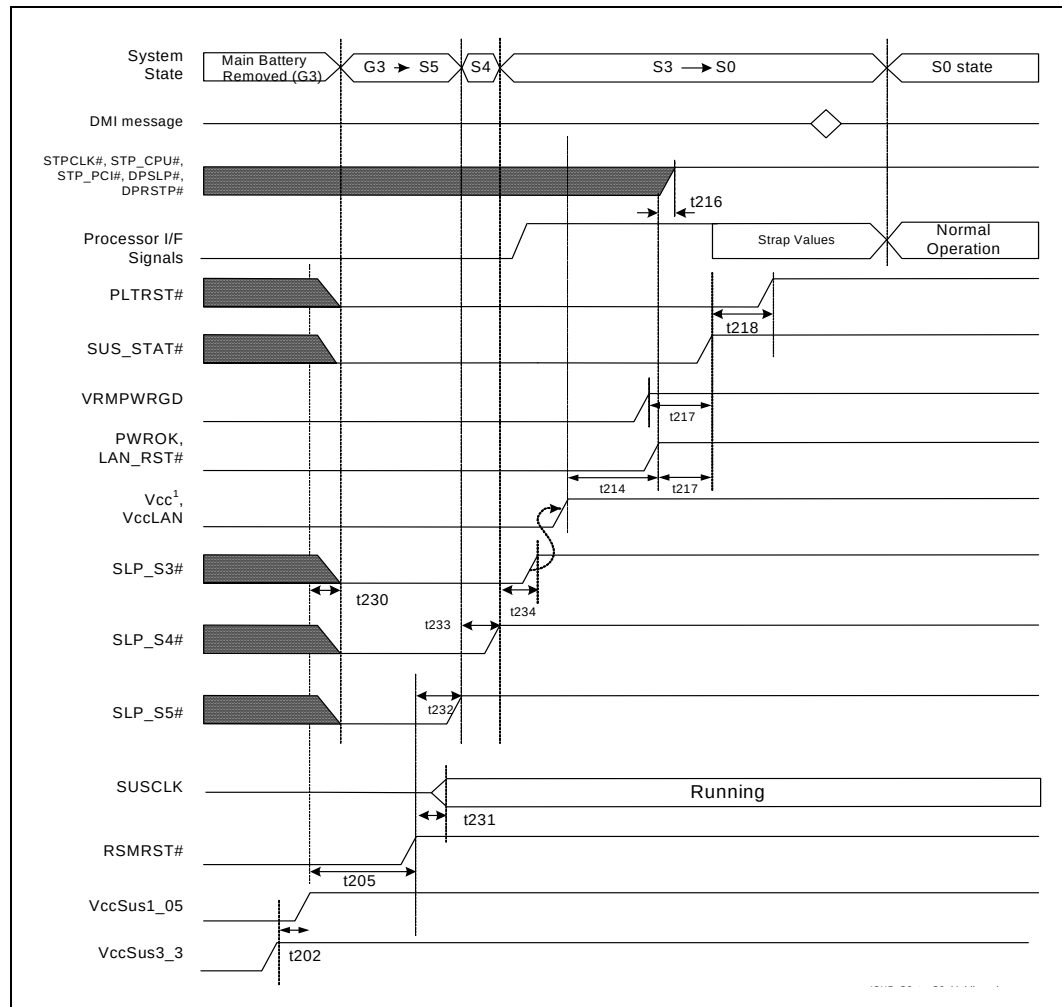
Figure 23-21. G3 (Mechanical Off) to S0 Timings (Mobile Only)
