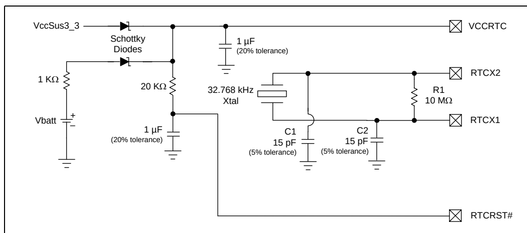
Figure 2-3. Example External RTC Circuit
