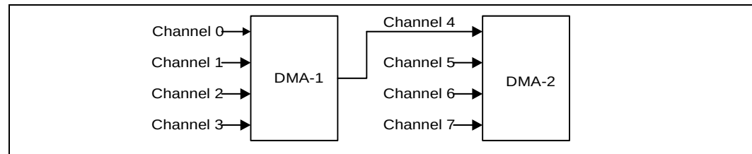
Figure 5-5. Intel® ICH7 DMA Controller
