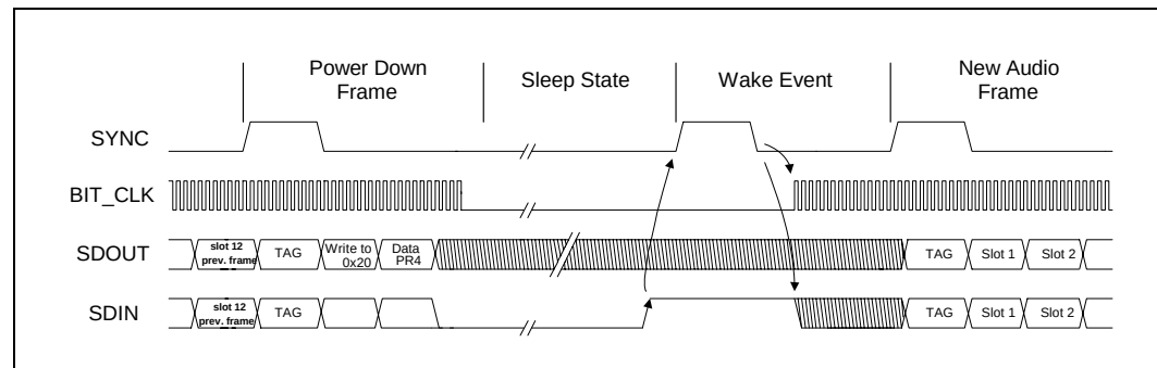
Figure 5-16. SDIN Wake Signaling
