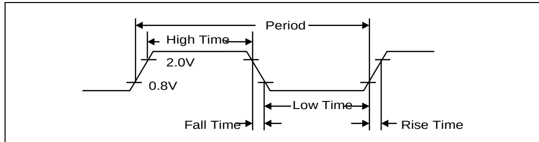
Figure 23-1. Clock Timing
