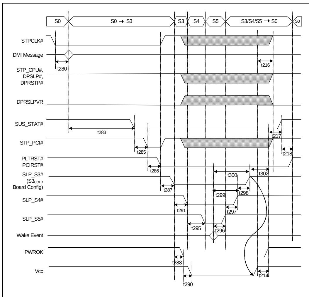
Figure 23-25. S0 to S5 to S0 Timings, S3 COLD (Mobile Only)
