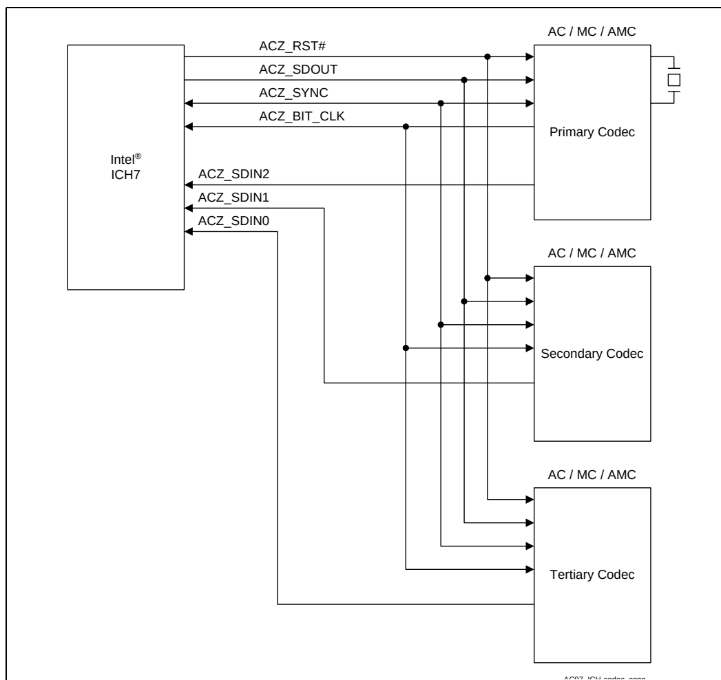
Figure 5-13. AC '97 2.3 Controller-Codec Connection
