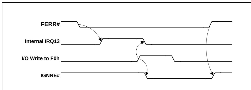
Figure 5-7. Coprocessor Error Timing Diagram
