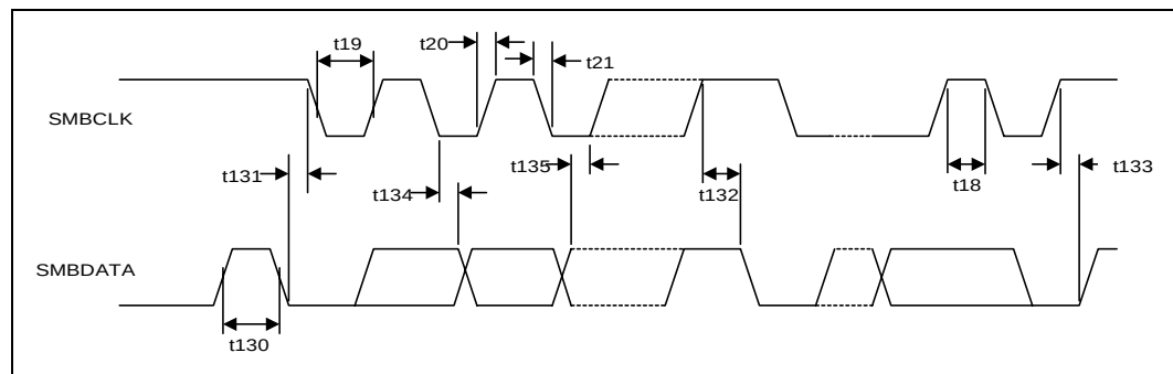
Figure 23-17. SMBus Timeout
