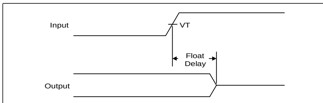
Figure 23-5. Pulse Width
