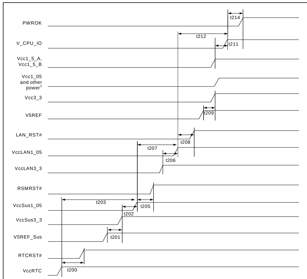
Figure 23-19. Power Sequencing and Reset Signal Timings (Mobile Only)
