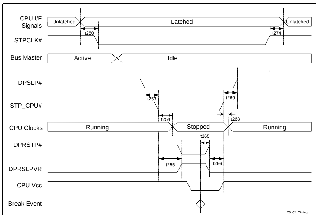
Figure 23-29. C0 to C4 to C0 Timings (Mobile Only)
