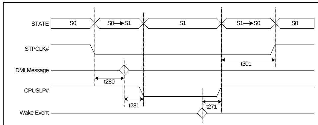
Figure 23-22. S0 to S1 to S0 Timing (Desktop Only)
