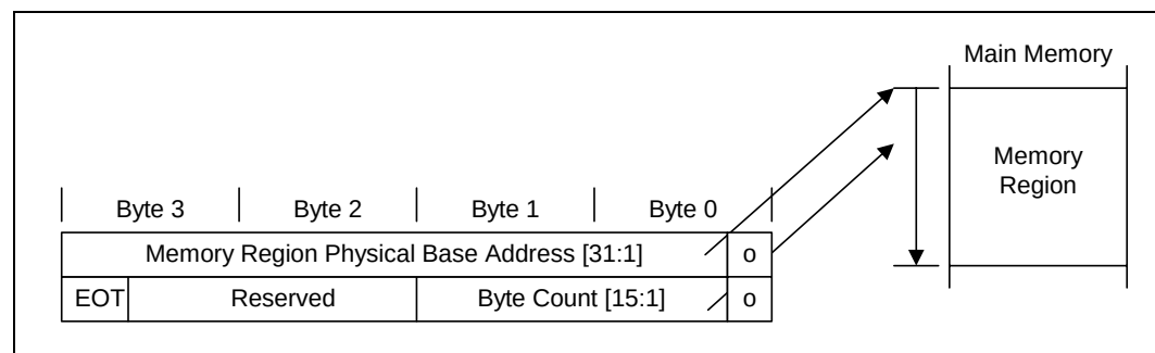
Figure 5-8. Physical Region Descriptor Table Entry
