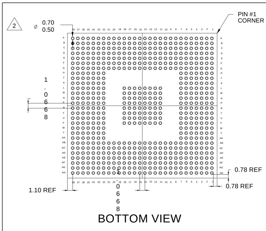
Figure 24-2. Intel® ICH7 Package (Bottom View)
