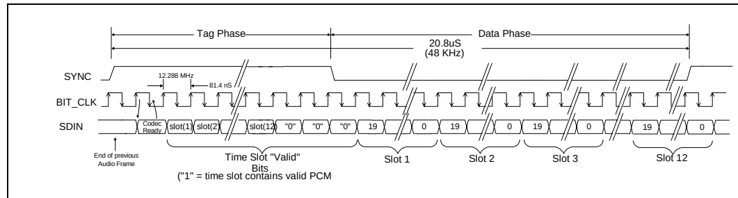
Figure 5-14. AC-Link Protocol
