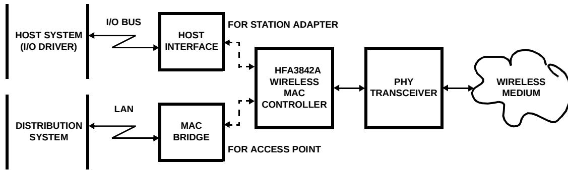
FIGURE 11. TYPICAL APPLICATION
