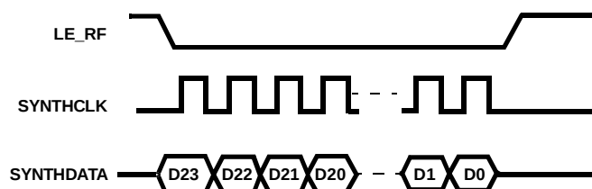
FIGURE 20. SYNTHESIZER DATA FORMAT
