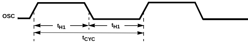
FIGURE 1. CLOCK SIGNAL TIMING
