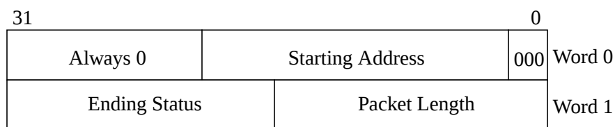
Figure 7. Ethernet Receive Descriptor
