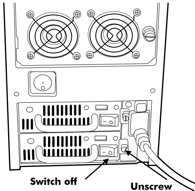
Figure : Swap P/S unit ( Unscrew )
