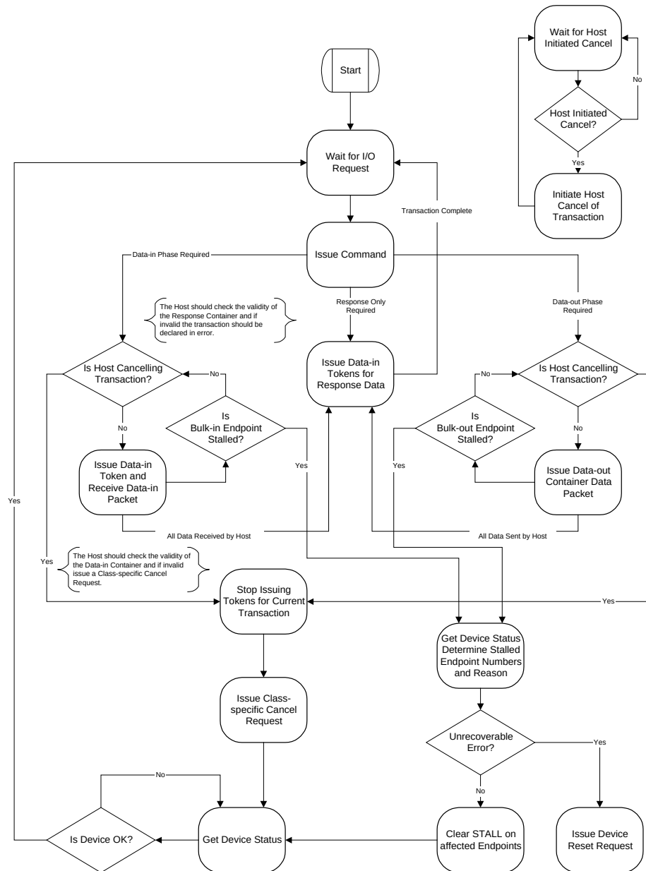
Figure 7.2-2 Still Image Protocol Host Behavior
