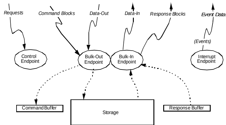
Figure 7.0-3 A USB Still Image Capture Device
