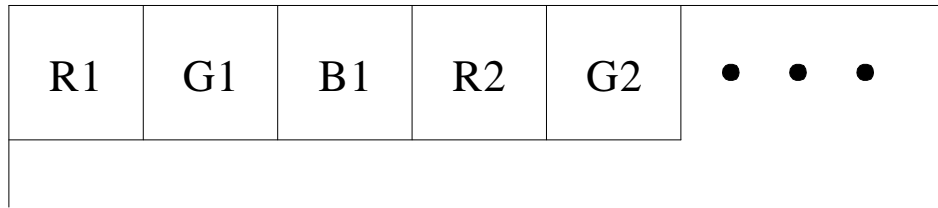
Figure 2.1.2: Pixel Data Map Representation
