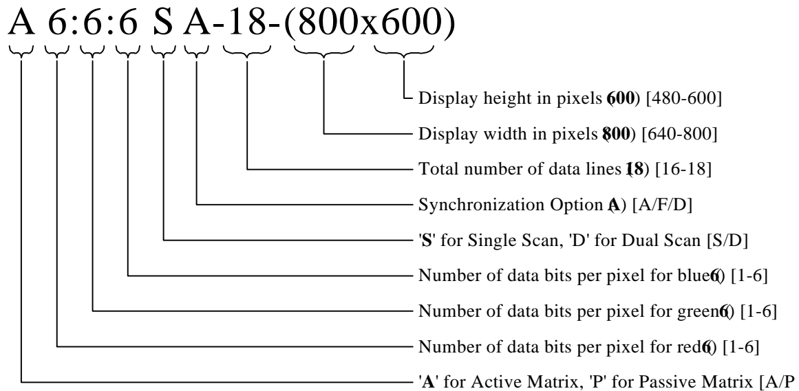
Figure 2.1.1: Panel Type Format Example
