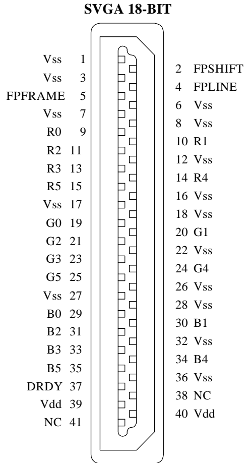
Figure 6.2.1: Recommended Active Matrix Pin Assignment (Plug Interface)
