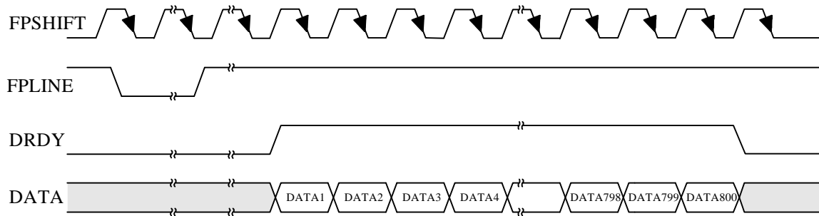
Figure 6.1.2.1: A6:6:6S-18-(800x600) Data Formatting
