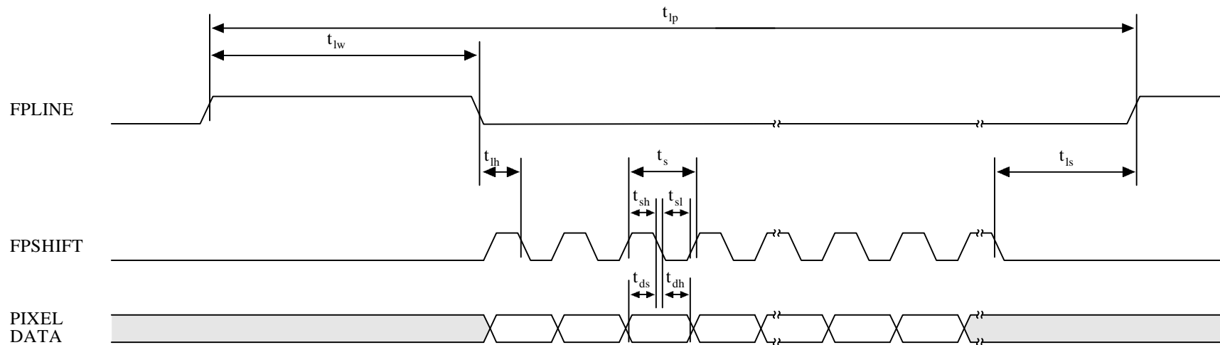
Figure 2.2.3.2a: P1:1:1D-16-(800x600) Horizontal Data Timing
