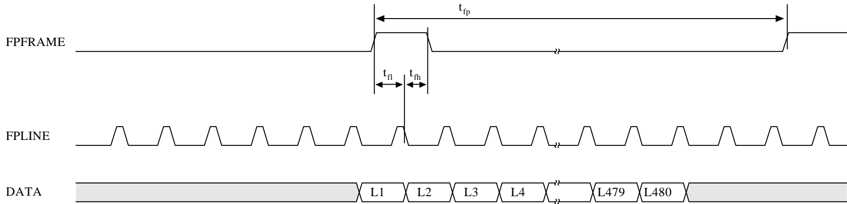
Figure 2.2.1.2b: P1:1:1S-16-(640x480) Vertical Data Timing
