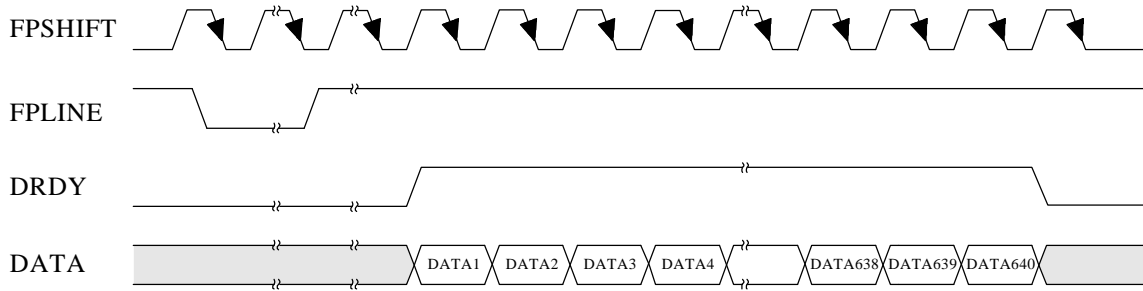
Figure 2.2.4.1: A3:3:3S-9-(640x480), A4:4:4S-12-(640x480), A6:6:6S-18-(640x480) Data Formatting
