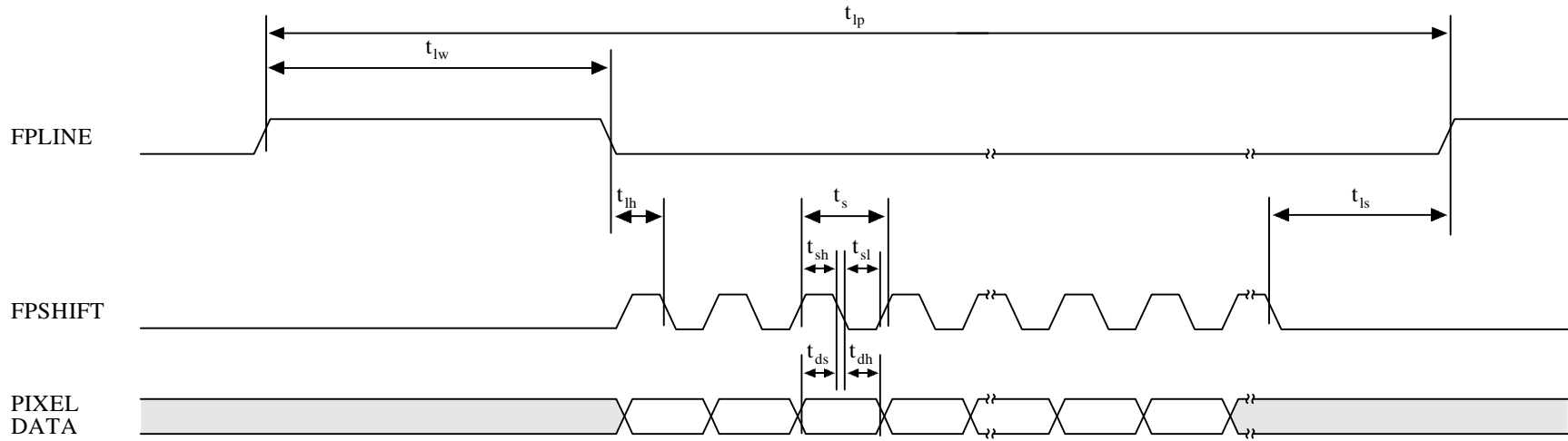
Figure 2.2.1.2a: P1:1:1S-16-(640x480) Horizontal Data Timing
