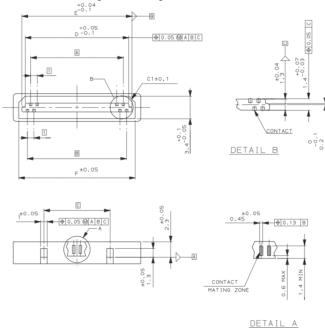
Figure 4.4.1: Plug Interface Dimensions
