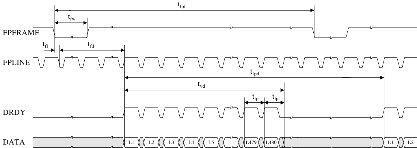
Figure 2.2.4.2b: A3:3:3S-9-(640x480), A4:4:4S-12-(640x480), A6:6:6S-18-(640x480) Vertical Data Timing
