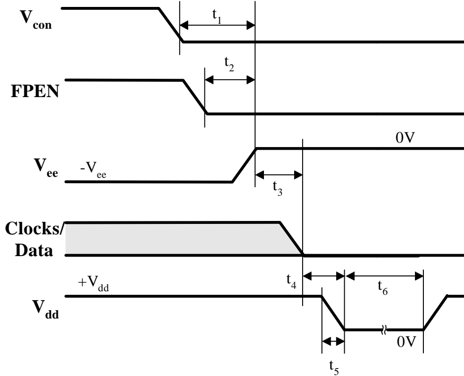
Figure 3.5.2: Power-down Sequencing
