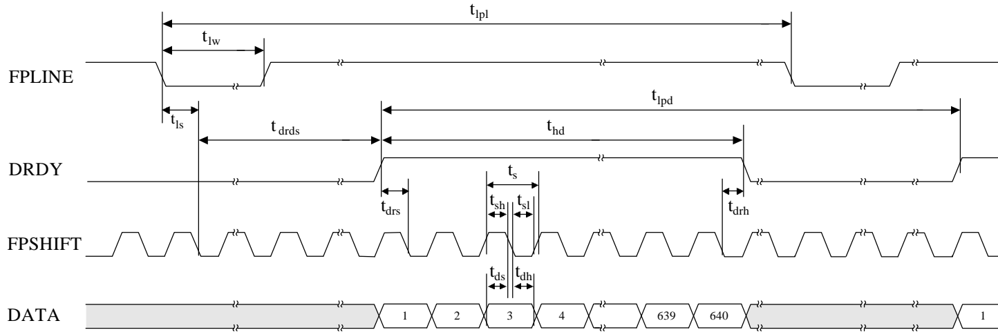
Figure 2.2.4.2a: A3:3:3S-9-(640x480), A4:4:4S-12-(640x480), A6:6:6S-18-(640x480) Horizontal Data Timing
