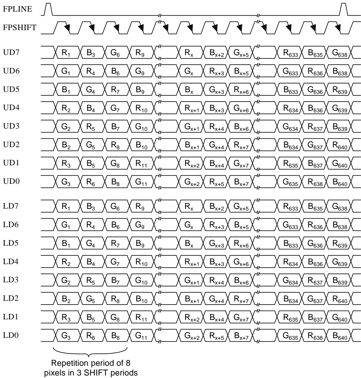
Figure 2.2.2.1: P1:1:1D-16-(640x480) Data Formatting
