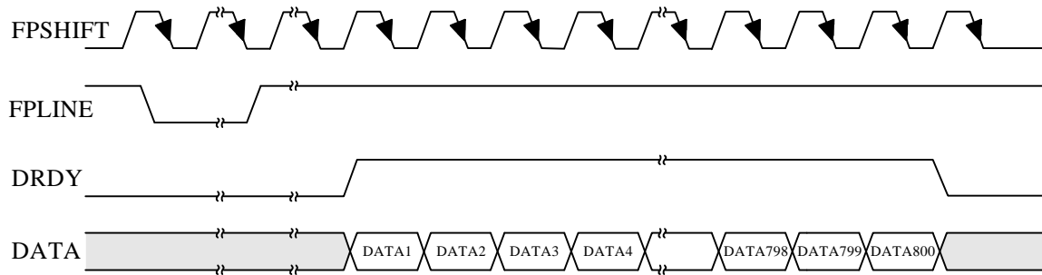
Figure 2.2.5.1: A4:4:4S-12-(800x600), A6:6:6S-18-(800x600) Data Formatting
