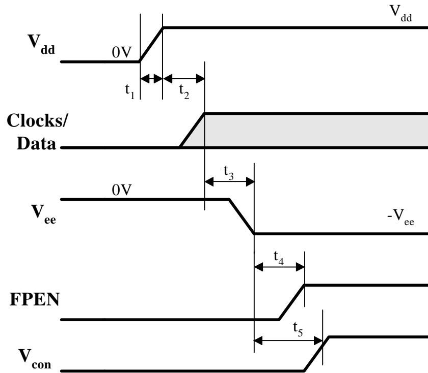
Figure 3.5.1: Power-up Sequencing
