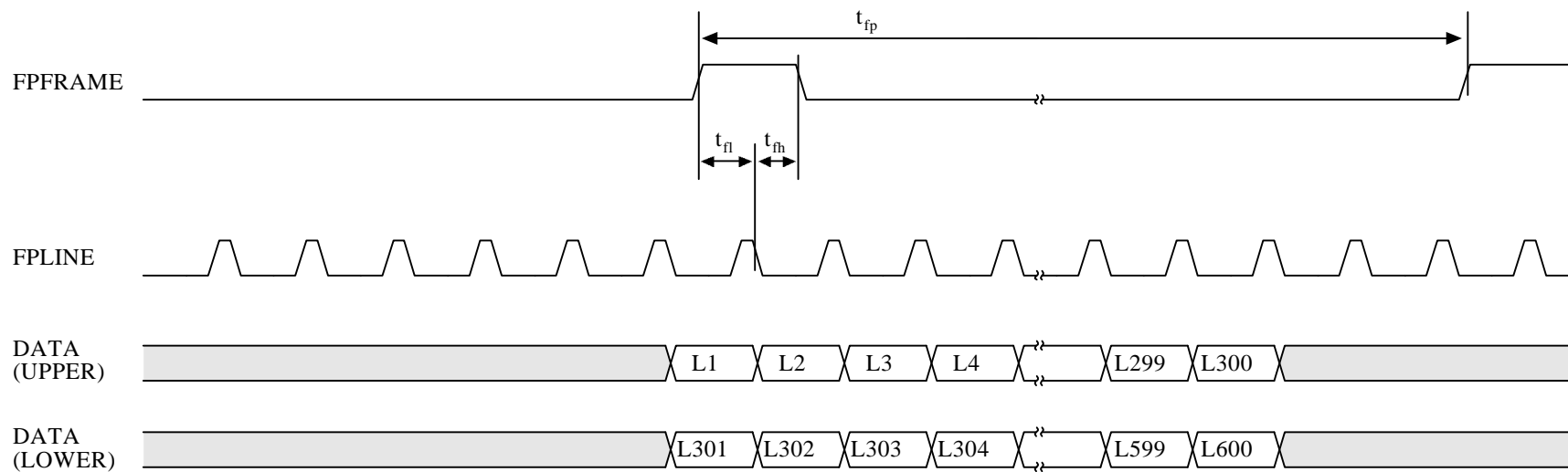
Figure 2.2.3.2b: P1:1:1D-16-(800x600) Vertical Data Timing
