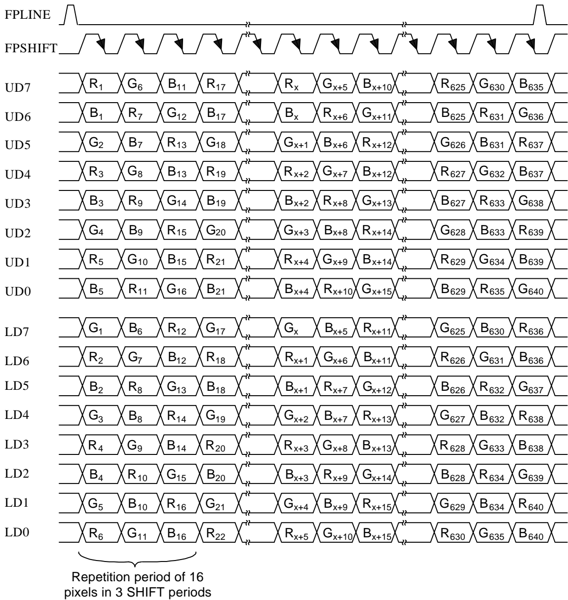
Figure 2.2.1.1: P1:1:1S-16-(640x480) Data Formatting
