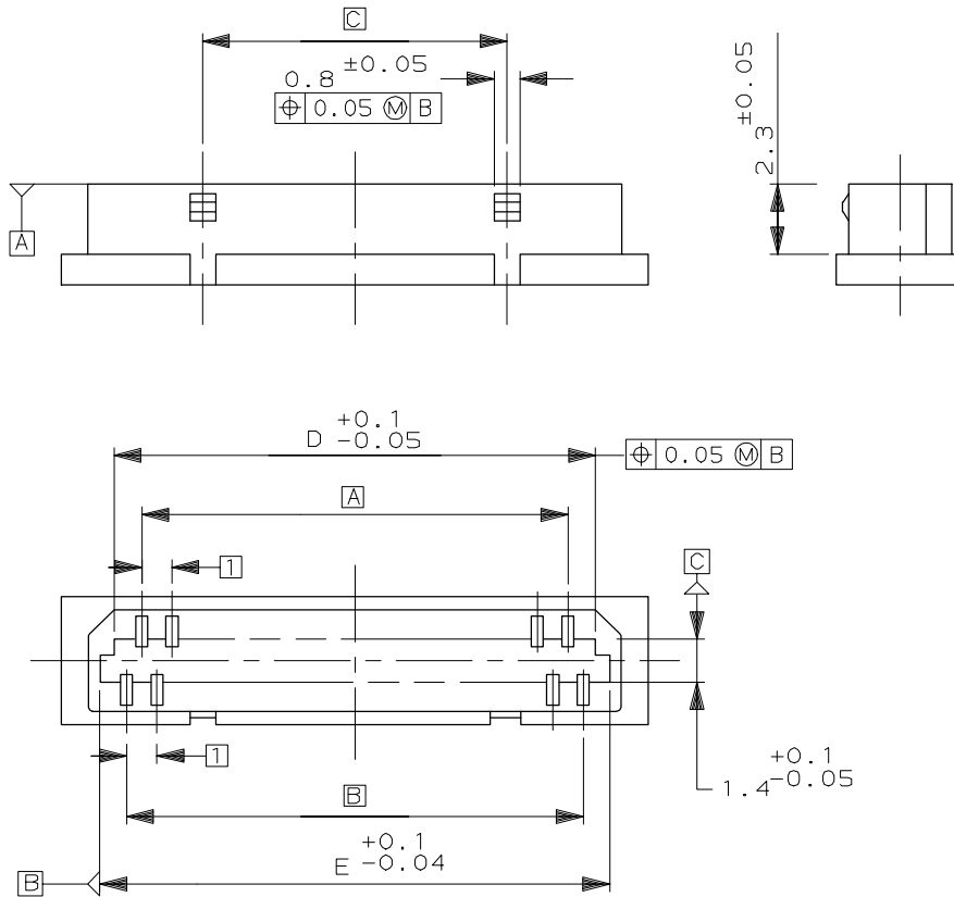
Figure 4.5.1: Receptacle Interface Dimensions
