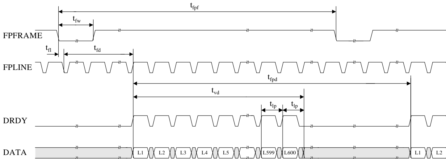
Figure 2.2.5.2b: A4:4:4S-12-(800x600), A6:6:6S-18-(800x600) Vertical Data Timing
