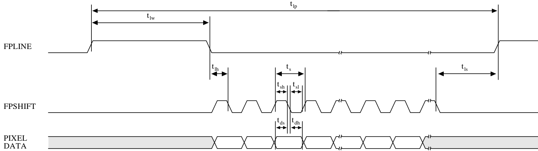
Figure 2.2.2.2a: P1:1:1D-16-(640x480) Horizontal Data Timing
