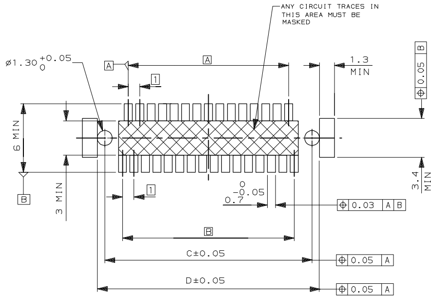
Figure 4.3.1: Recommended PCB Layout
