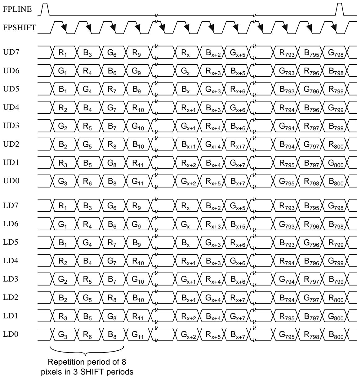
Figure 2.2.3.1: P1:1:1D-16-(800x600) Data Formatting
