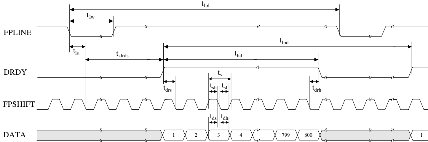
Figure 2.2.5.2a: A4:4:4S-12-(800x600), A6:6:6S-18-(800x600) Horizontal Data Timing
