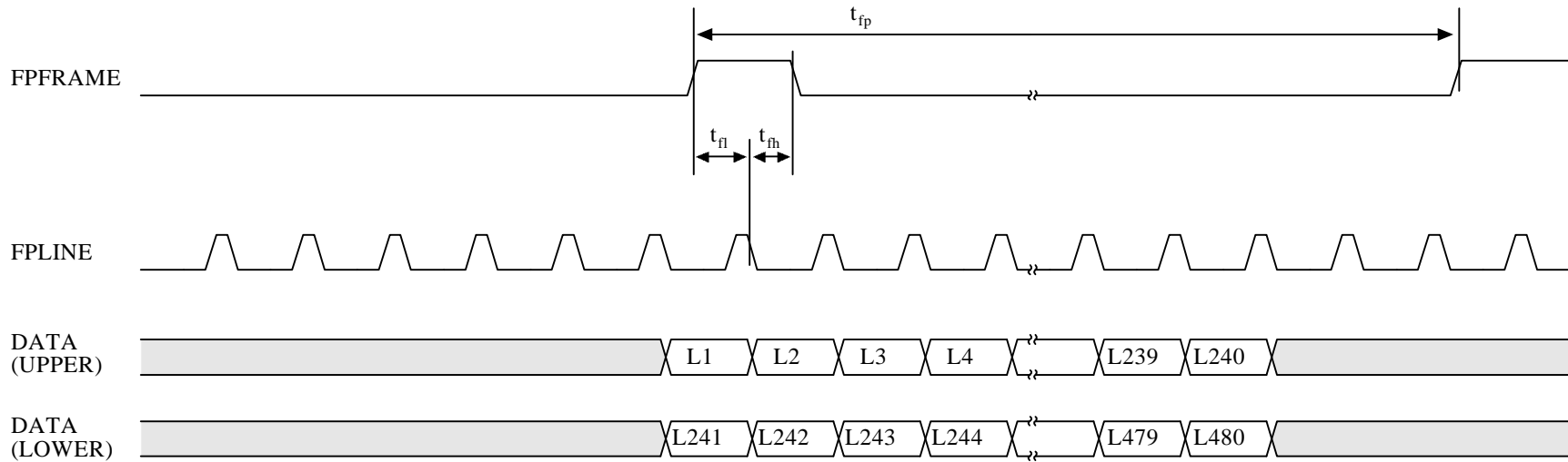
Figure 2.2.2.2b: P1:1:1D-16-(640x480) Vertical Data Timing
