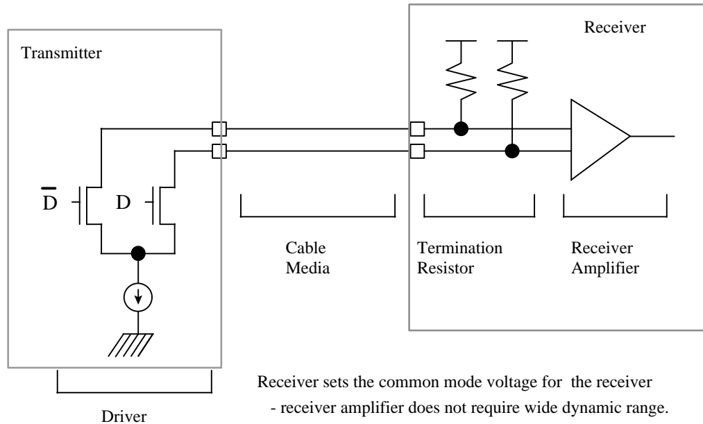
Figure 3-6: Typical CMOS Circuits for TMDS Driver
