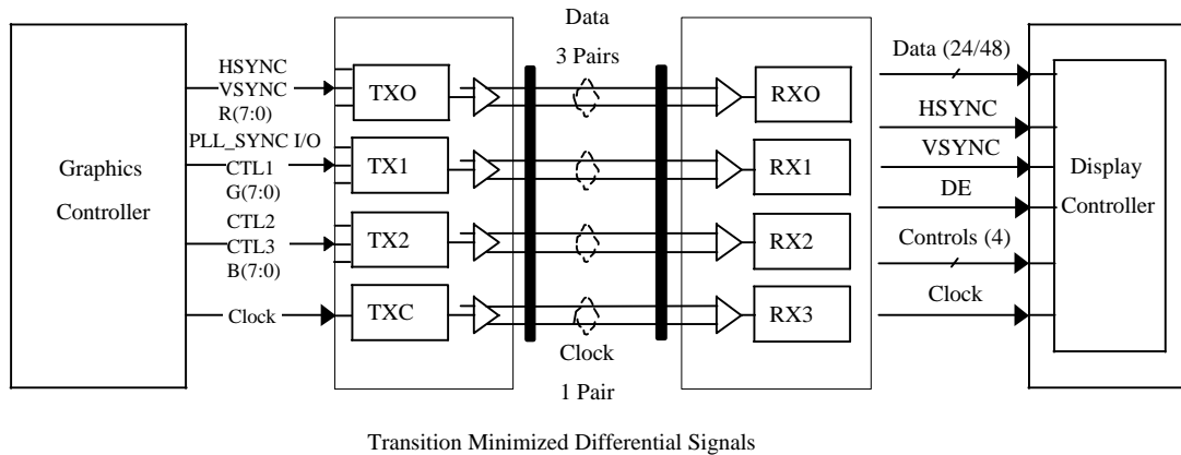
Figure 3-4: System Environment Block Diagram Example
