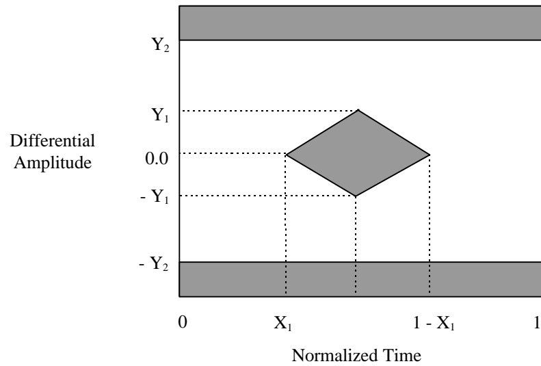
Figure 8-9: Eye Diagram Mask at Point R
