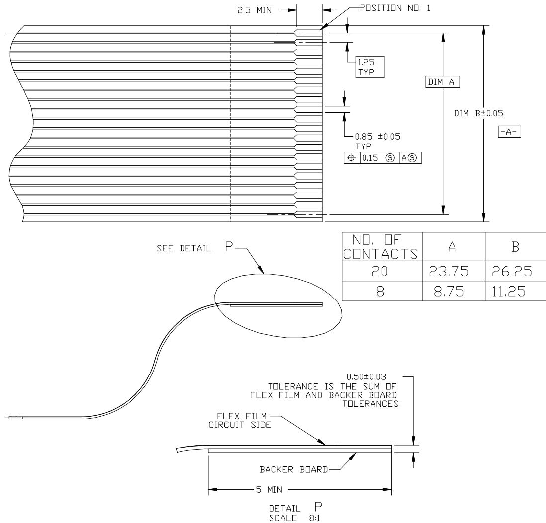
Figure 7-4: Recommended FEC Mating Interface Features
