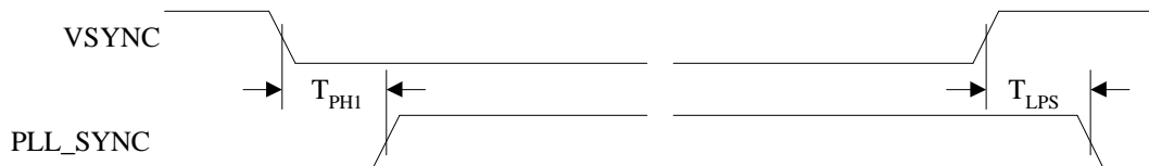
Figure 8-18. PLL_SYNC Timing of Transmitter with SYNC_CONT = 1
