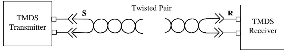
Figure 8-7: TMDS Connection
