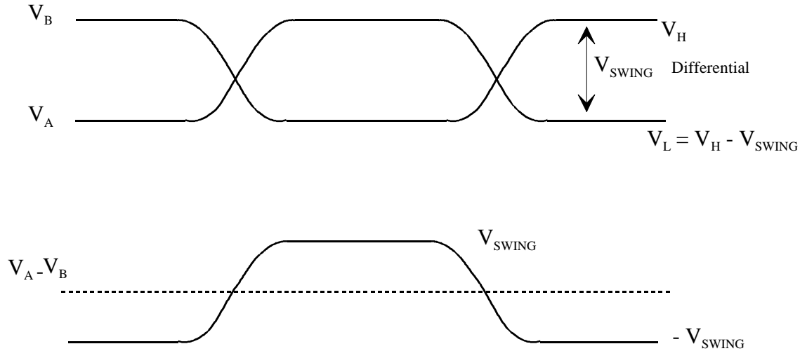
Figure 8-2: Signal Levels on Transmission Media
